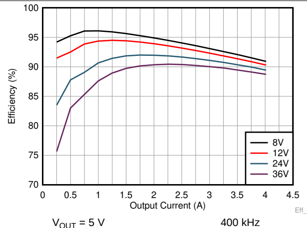
Figure 12. High-Load Efficiency
