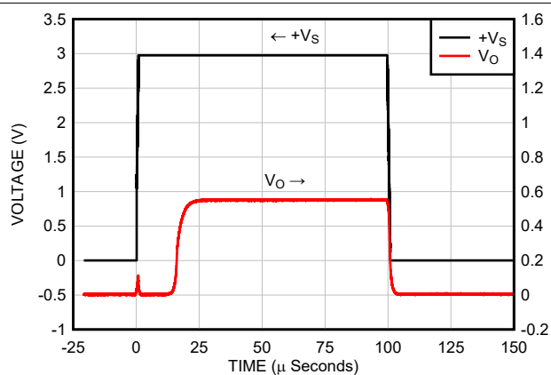
図 6-20. Start-Up Response (New chip)
