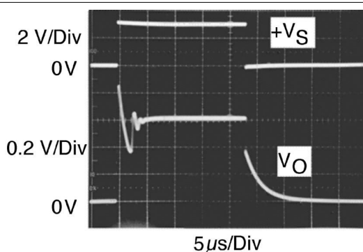
図 6-19. Start-Up Response (Legacy chip)
