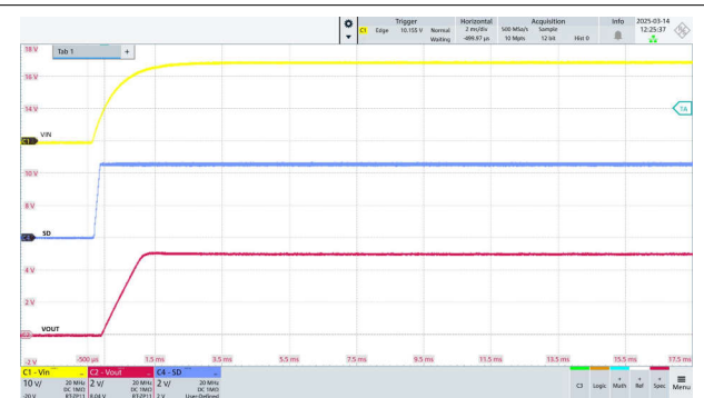
図 7-11. Start-Up Operation
