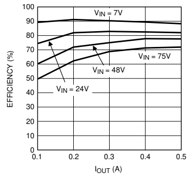
FIG 5-7. Demoboard Efficiency vs I_{OUT} and V_{IN}
