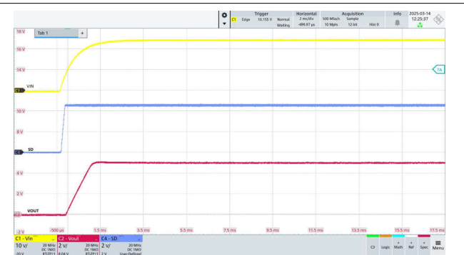
図 7-11. Start-Up Operation
