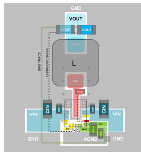
11-2. Recommended Layout for LM53625/35-Q1
