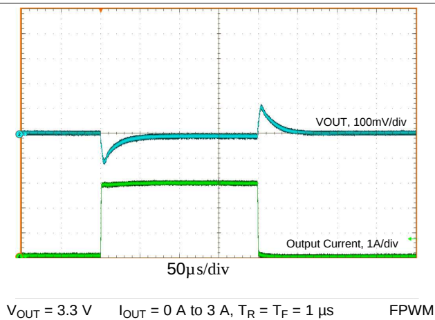
Figure 43. Load Transient
