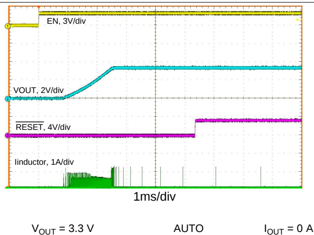
Figure 41. Start-Up
