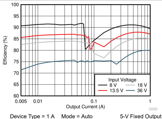
9-5. Efficiency
