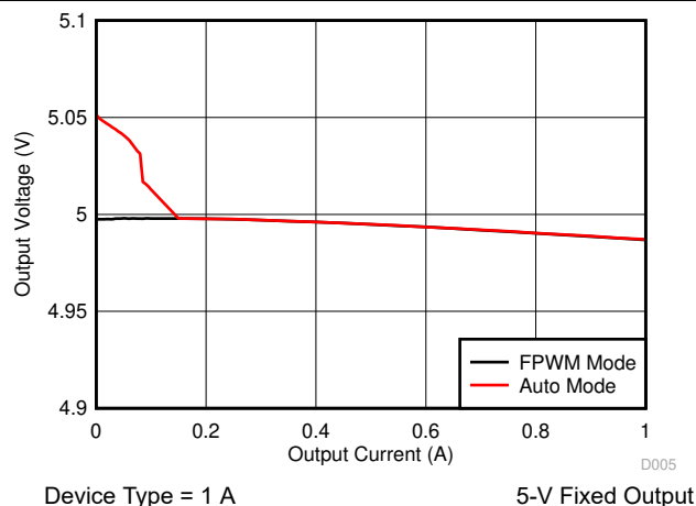
9-6. Load Regulation
