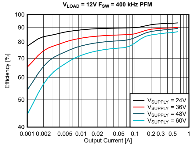
7-6. PFM Mode Efficiency, Log Scale
