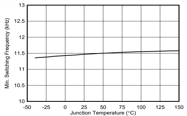
図 6-12. Minimum Switching Frequency versus Temperature
