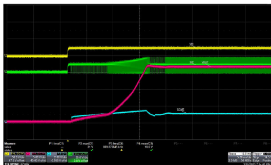
図 8-4. Start-Up Characteristic at No Load
