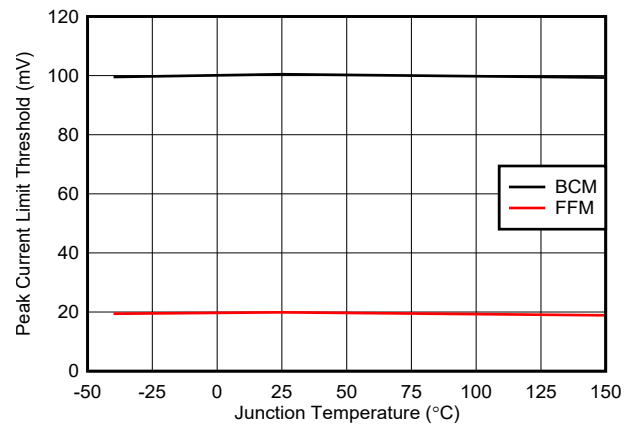
図 6-10. Peak Current Limit Thresholds vs. Temperature
