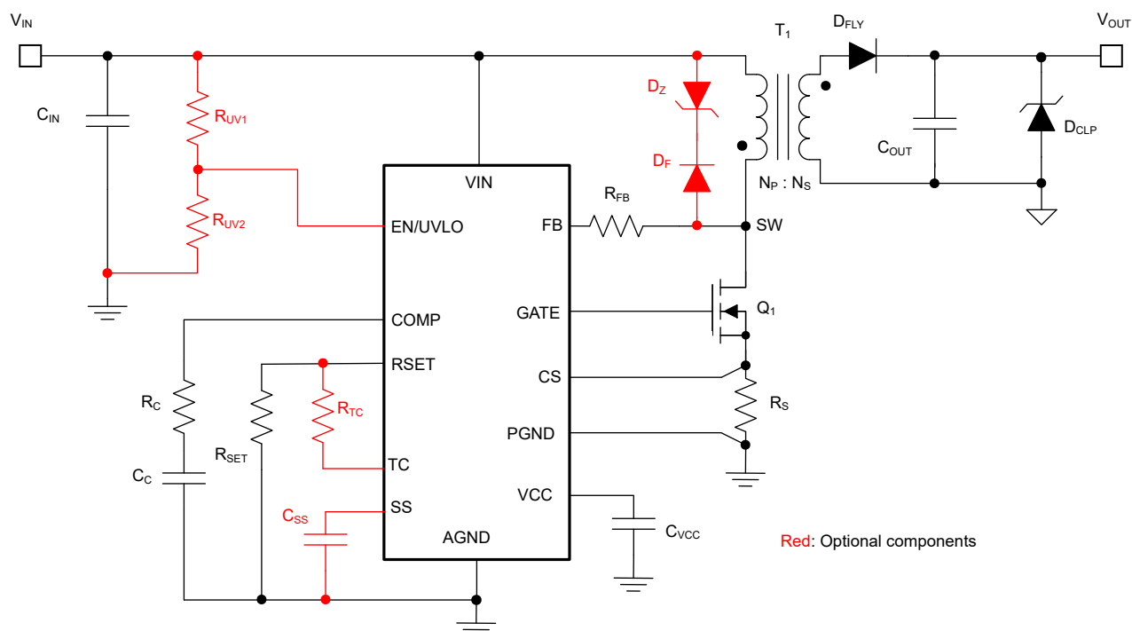
7-1. LM5185-Q1 Flyback Converter Schematic (Optional Components in Red)
