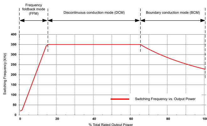
7-2. Three Modes of Operation Illustrated by Variation of Switching Frequency With Load
