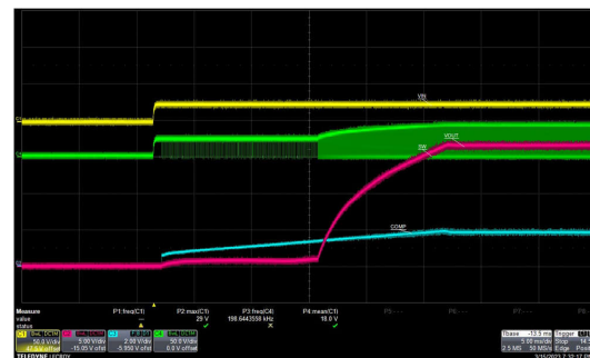
図 8-5. Start-Up Characteristic at Full Load
