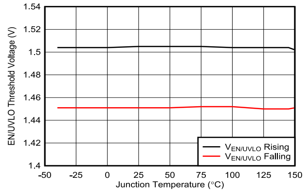
図 6-8. EN/UVLO Threshold Voltages versus Temperature
