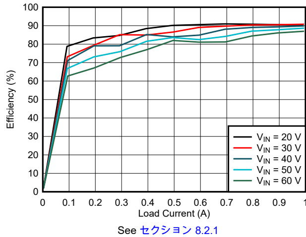
図 6-1. Efficiency versus Load
