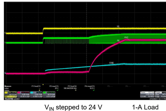
図 8-5. Start-Up Characteristic at Full Load
