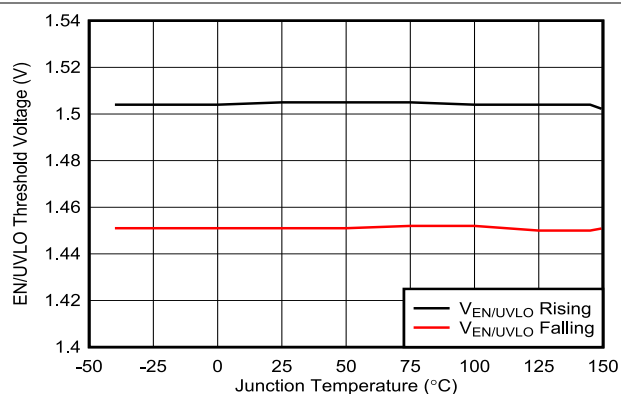
図 6-8. EN/UVLO Threshold Voltages versus Temperature
