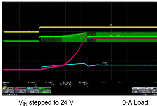
図 8-4. Start-Up Characteristic at No Load
