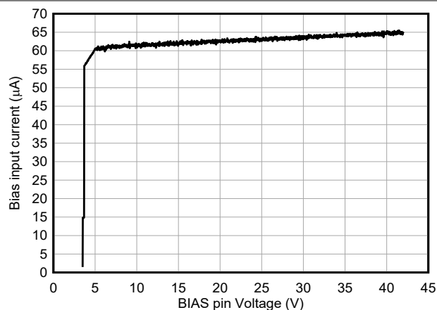
FIG 5-19. Quiescent Current into BIAS versus Pin Voltage V_{EN/UVLO} = 3.3\text{ V} , V_{(VIN)} = 12\text{ V}
