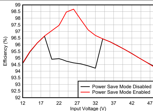
図 8-15. Efficiency Versus V_{IN} ( V_O = 24\text{ V} , I_O = 5\text{ A} )
