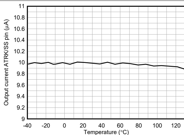
FIG 5-21. Soft-Start current versus Temperature
