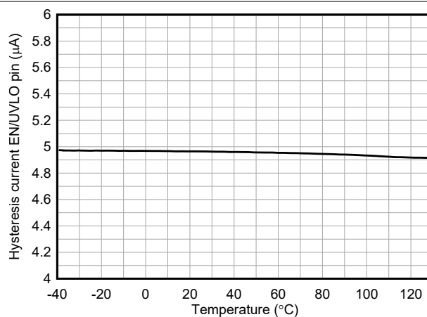
FIG 5-22. Hysteresis Current on EN/UVLO versus Temperature
