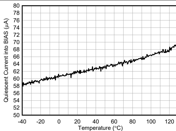
FIG 5-20. Quiescent Current into BIAS versus Temperature V_{EN/UVLO} = 3.3\text{ V} , V_{(VIN)} = 12\text{ V}
