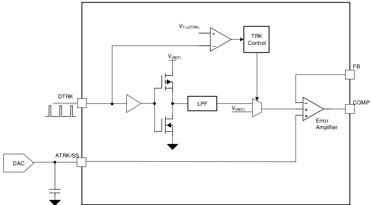
7-14. Output Voltage Tracking Functional Block Diagram
