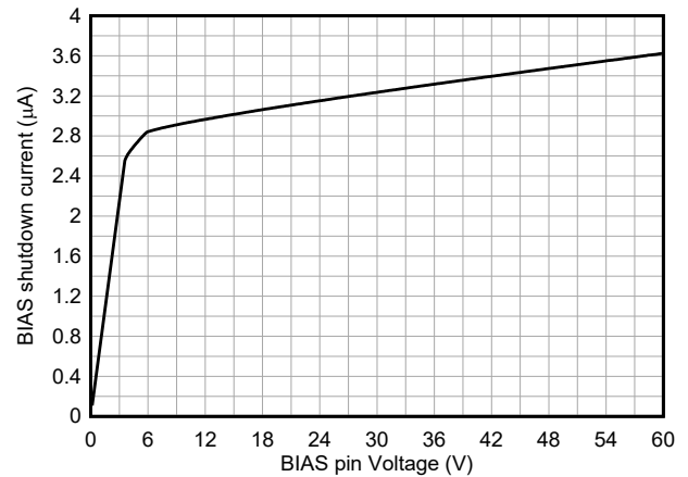
FIG 5-16. Shutdown Current into BIAS versus Pin Voltage V_{EN/UVLO} = 0\text{ V} , V_{(VIN)} = 12\text{ V} , V_{(VIN)} = 3.5\text{ V}
