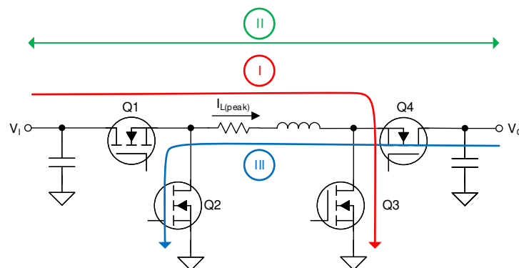
7-1. Buck-Boost Active Switching States
