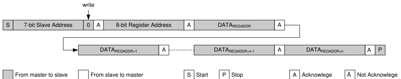
図 6-39. Sequential WRITE Starting At A Defined Register Address
