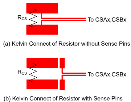
図 7-35. A Layout Example of Current Sense Routing
