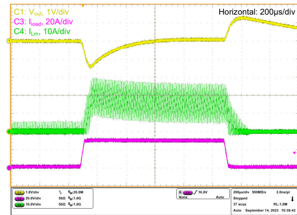
7-17. Step Load Response: Buck Mode; DEM; 1A to 30A Load Step; 1A/μs
