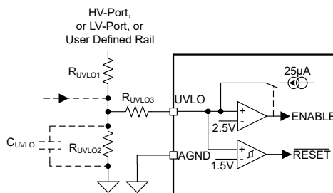
6-32. UVLO With Additional Hysteresis Programming
