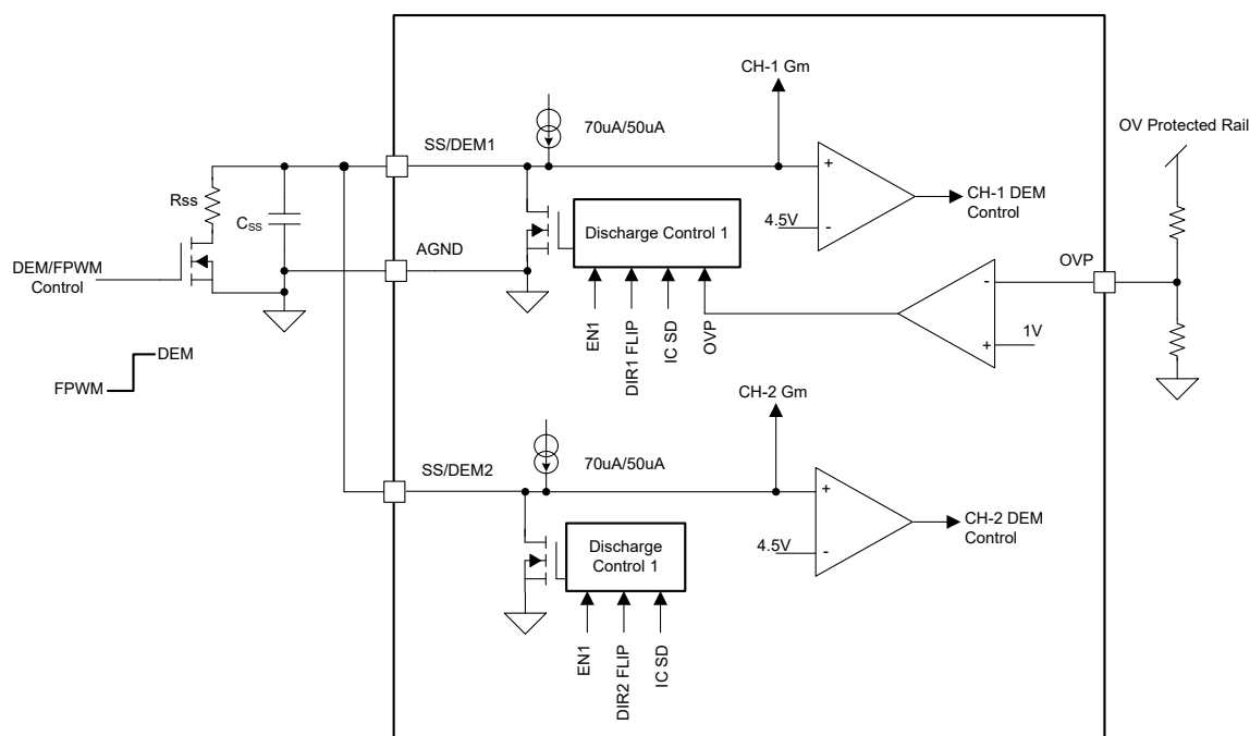
6-12. OVP Implementation for SS-DEM Pins Connection for Parallel Operation
