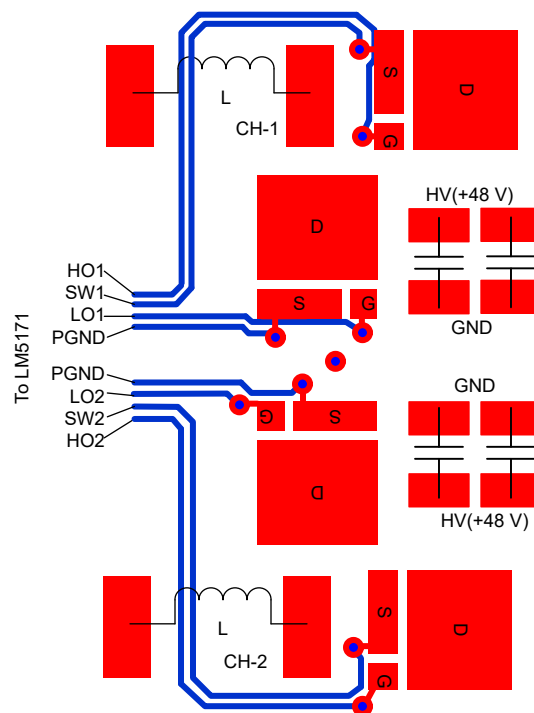
図 7-34. A Layout Example of MOSFET Gate Drive Routing
