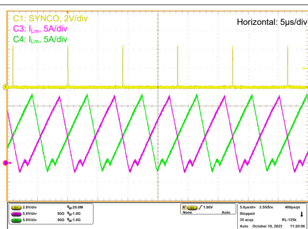
図 7-20. Dual-Channel Interleaving Operation: Boost Mode, I_{load} = 4A
