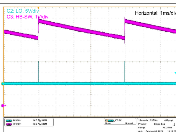
図 7-29. Pre-charge: Buck Mode, I_{load} = 0A
