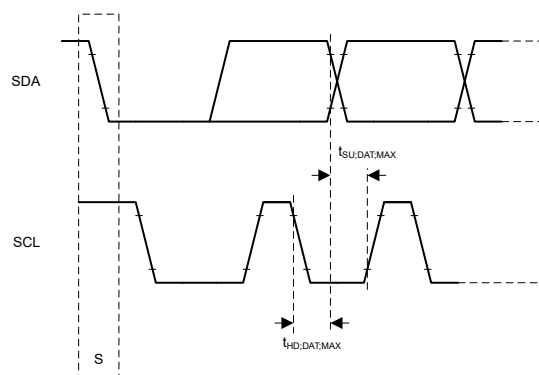
図 6-35. I 2 C Data Transmission Timing for maximum rise/fall times.
