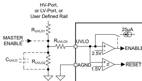
6-31. UVLO Programming
