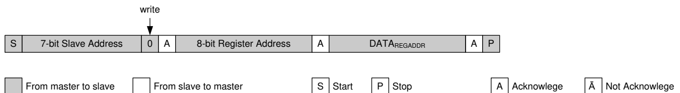
図 6-38. Single WRITE to Defined Register Address
