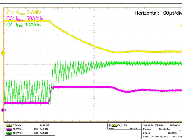
図 7-31. Output Short Circuit: Buck Mode
