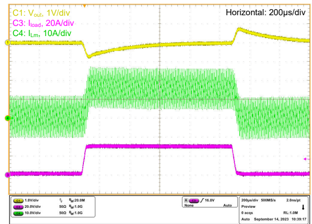
7-18. Step Load Response: Buck Mode; FPWM; 1A to 30A Load Step; 1A/μs
