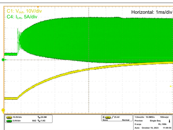
図 7-22. Start Up: Boost Mode, I_{load} = 4A
