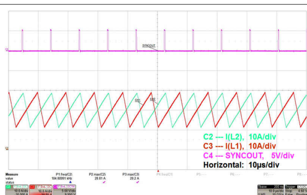
9-21. Dual-Channel Interleaving Operation: Boost Mode
