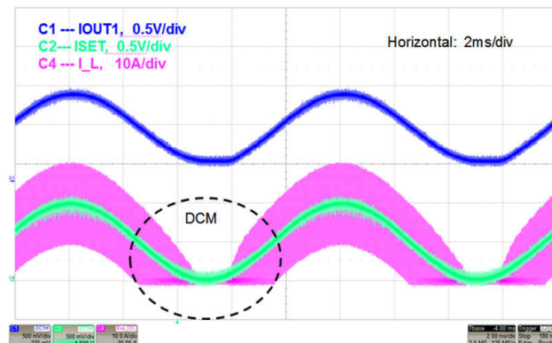
图 9-15. Diode Emulation Prevents Negative Current
