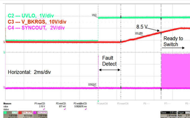
图 9-17. Start-Up Sequence Following UVLO Enable
