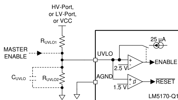
Figure 8-28. UVLO Programming
