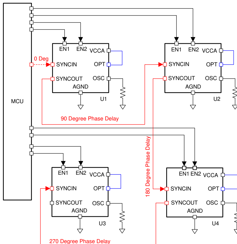
FIG 8-25. Eight Phases 90° Interleaving Configuration
