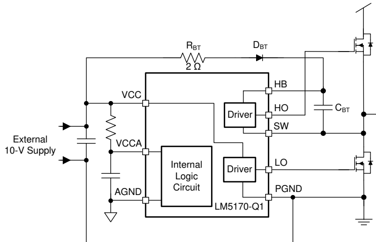
FIG 8-8. Bootstrap Circuit for High-Side Bias Supply
