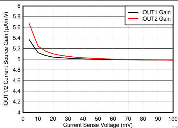
7-6. IOUT1/2 Current Monitor Accuracy vs V_{CS}
