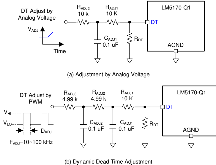
8-27. Dynamic Dead Time Adjustment
