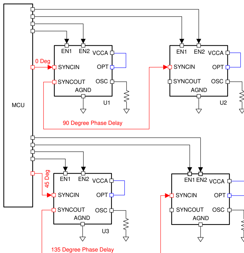
FIG 8-24. Eight Phases 45° Interleaving Configuration
