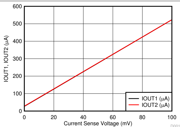
7-9. IOUT1/2 Current Monitor vs V_{CS} Voltage
