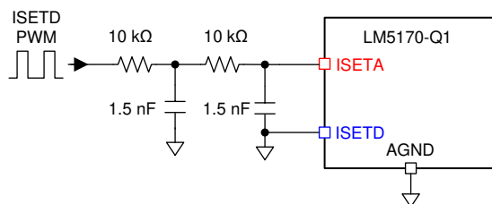
Figure 9-13. Two-Stage RC Filter to Convert the PWM into an Analog Voltage at the ISETA Pin
