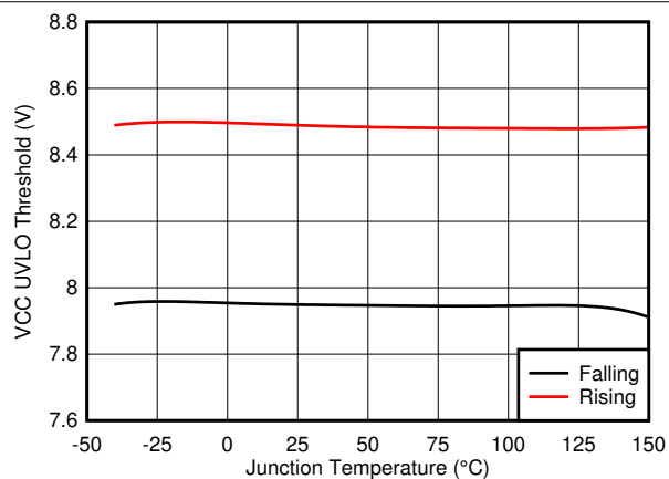
7-4. VCC UVLO Threshold vs Temperature
