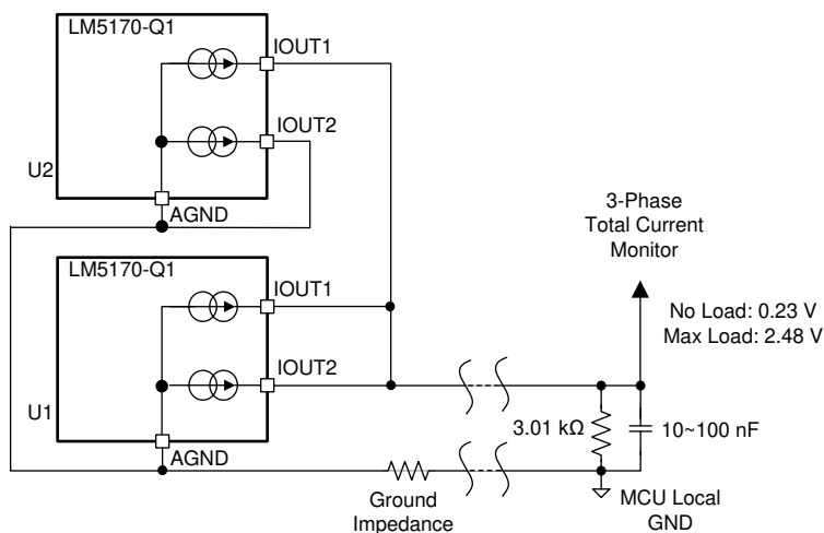
FIG 8-26. 3-Phase Total Current Monitor
