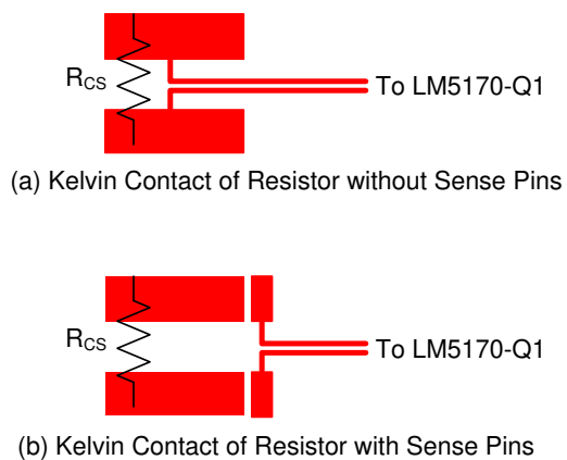
11-3. A Layout Example of Current Sense Routing
