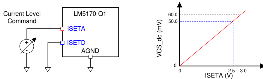
8-3. Pin Configurations for Current Setting Using an Analog Voltage Signal
