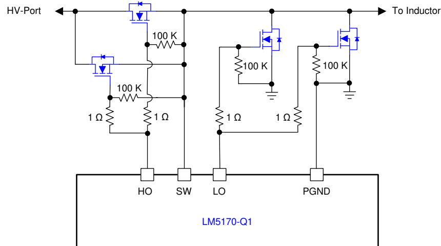
FIG 9-10. Paralleled MOSFET Configuration
