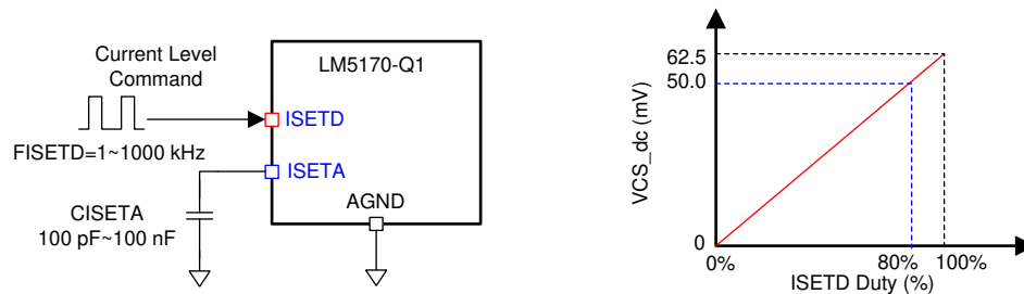
8-4. Pin Configurations for Current Setting Using a PWM Signal
