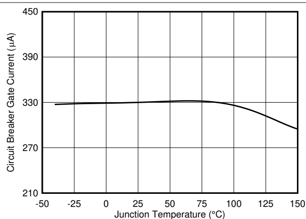
7-18. Circuit Breaker Gate Current vs Temperature
