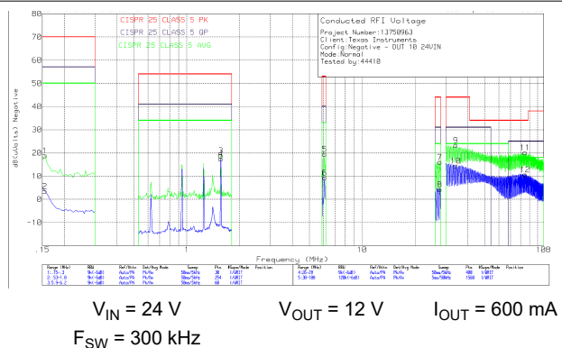
9-37. Conducted EMI (Negative Rail)
