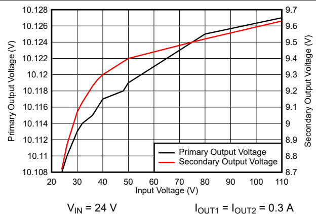
FIG 9-5. Line Regulation
