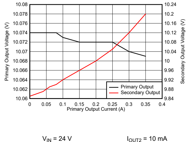
FIG 9-3. Load Regulation vs Primary Load Current
