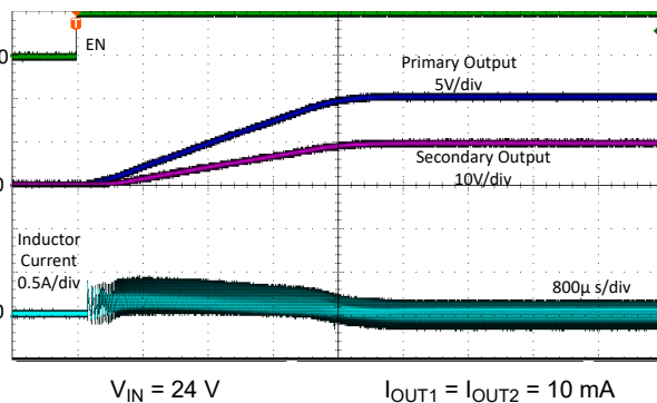
FIG 9-6. Light Load Start-Up from EN
