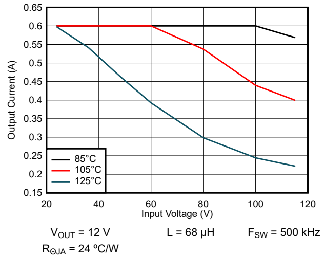
9-35. Maximum Output Current: VOUT = 12 V
