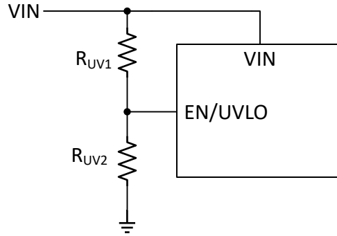
8-2. Input UVLO Connections
