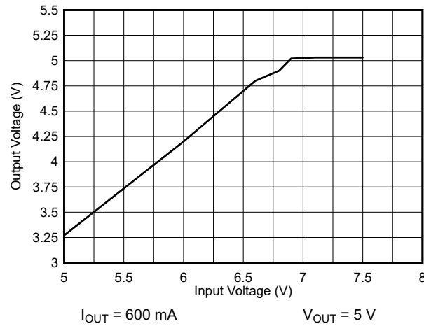
9-31. Drop-Out Response
