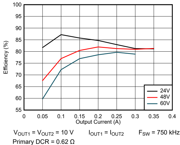
FIG 9-2. Efficiency
