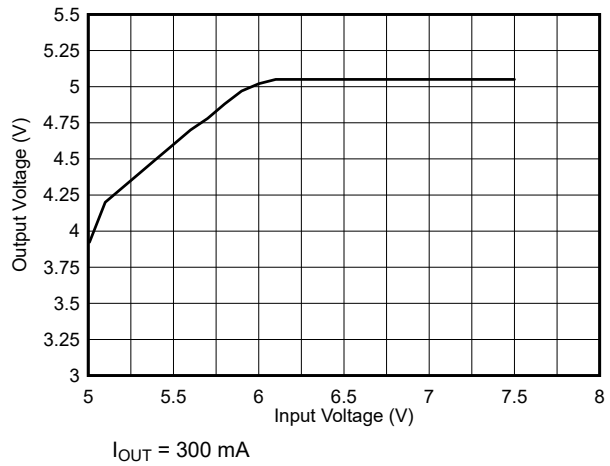
9-32. Drop-Out Response
