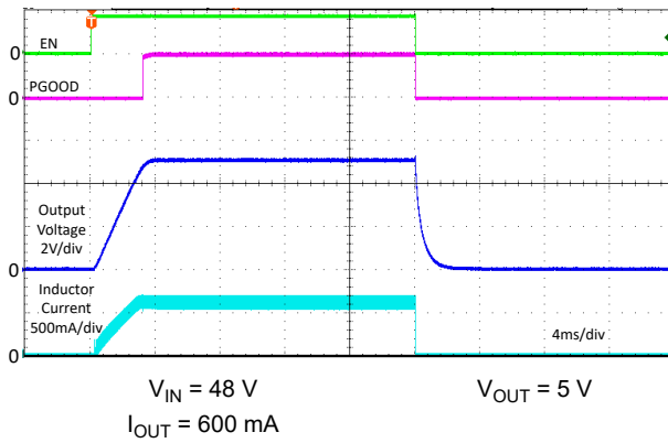
9-29. Typical Start-up Waveforms
