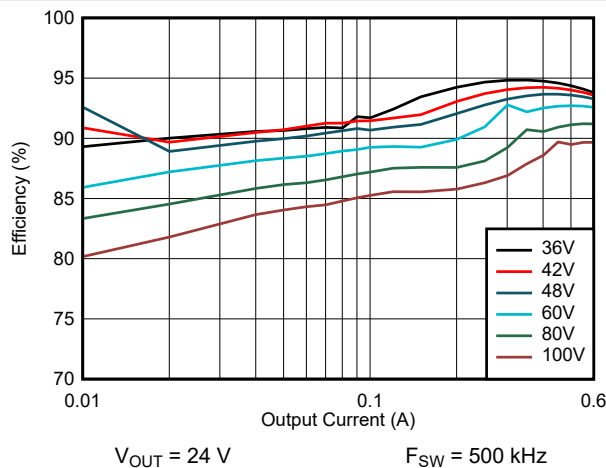
FIG 9-17. Efficiency: V_{OUT} = 24\text{ V}
