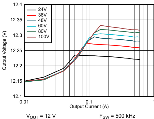
FIG 9-19. Line and Load Regulation: V_{OUT} = 12\text{ V}
