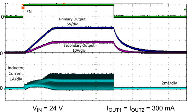
FIG 9-7. Full Load Start-Up from EN
