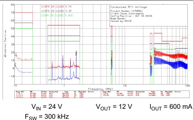
9-36. Conducted EMI (Positive Rail)
