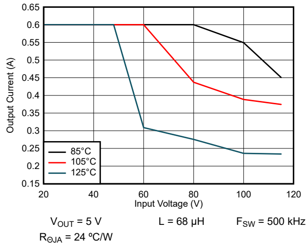
9-34. Maximum Output Current: VOUT = 5 V
