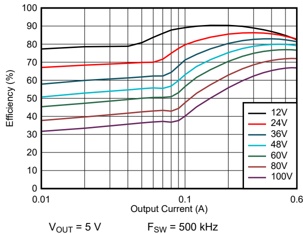
FIG 9-15. Efficiency: V_{OUT} = 5\text{ V}
