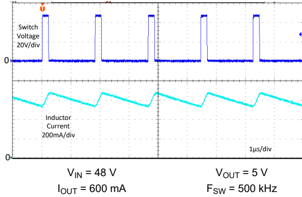
9-27. Typical Switching Waveforms
