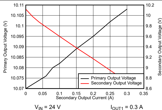
FIG 9-4. Load Regulation vs Secondary Load Current
