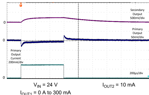
8-8. Load Transient on Primary Output
