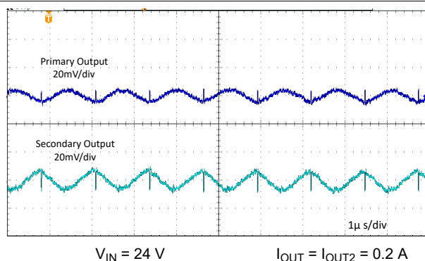
8-13. Typical Output Ripple
