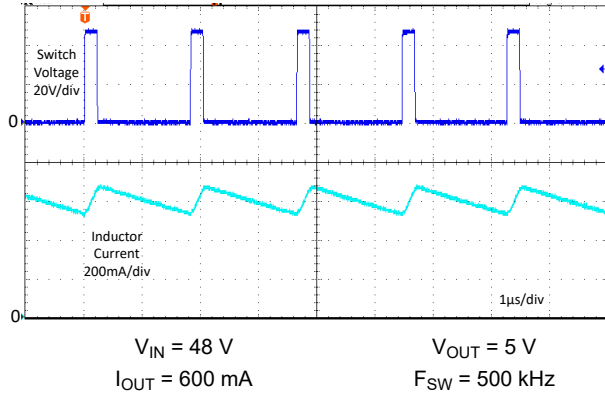
8-27. Typical Switching Waveforms
