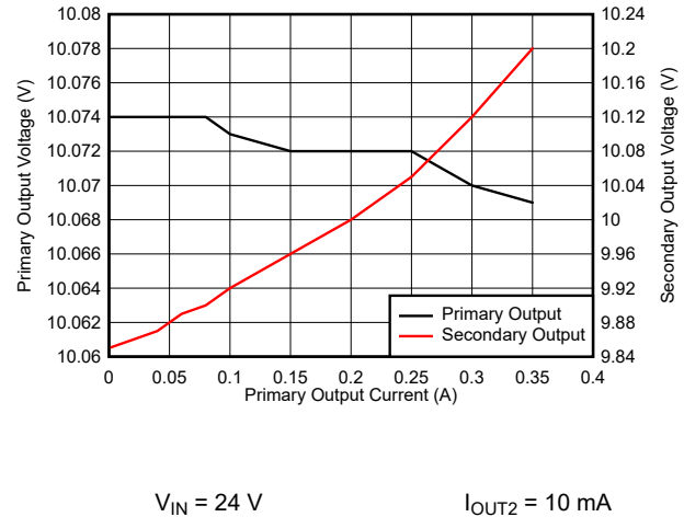
図 8-3. Load Regulation vs Primary Load Current
