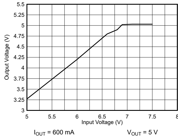
8-31. Drop-Out Response
