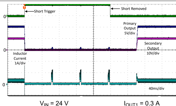
8-11. Short Circuit on Secondary Output
