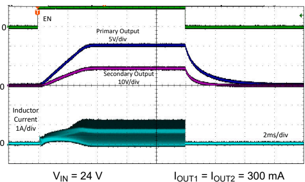
図 8-7. Full Load Start-Up from EN
