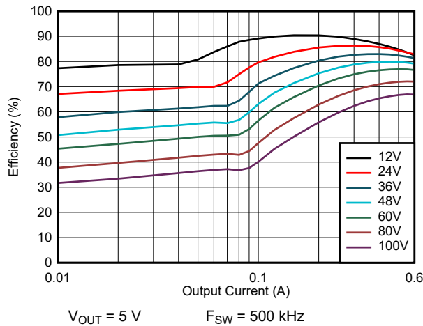
図 8-15. Efficiency: V_{OUT} = 5\text{ V}
