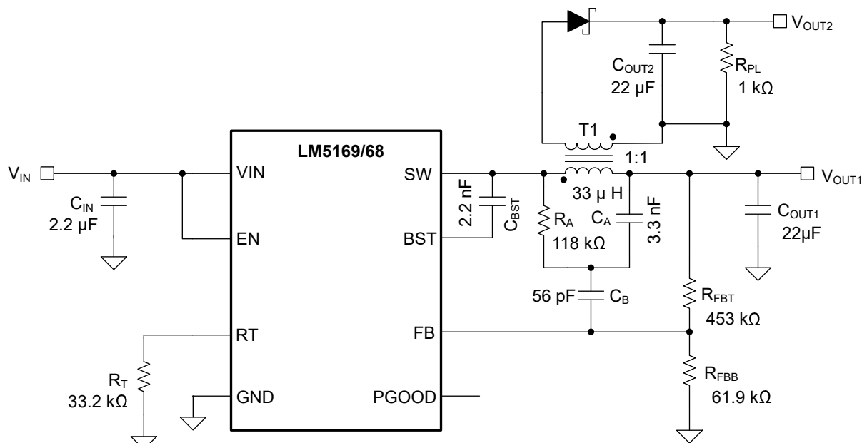
8-1. Example Fly-Buck™ Converter Application Circuit
