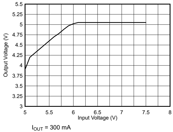
8-32. Drop-Out Response
