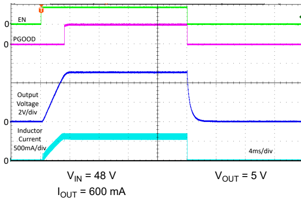
8-29. Typical Start-up Waveforms
