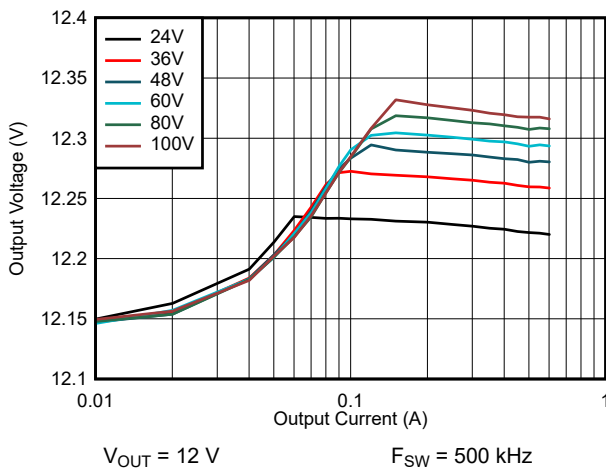
図 8-19. Line and Load Regulation: V_{OUT} = 12\text{ V}
