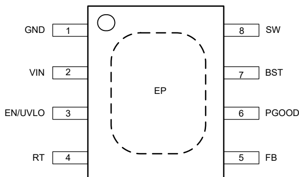
図 5-1. 8-Pin SO PowerPAD™ Integrated Circuit Package (Top View)
