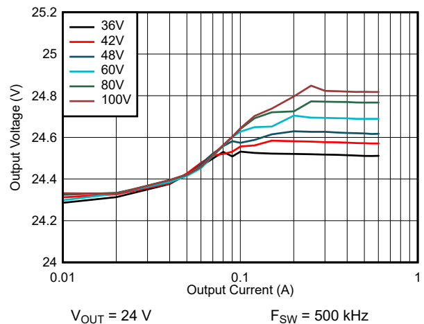
図 8-20. Line and Load Regulation: V_{OUT} = 24\text{ V}
