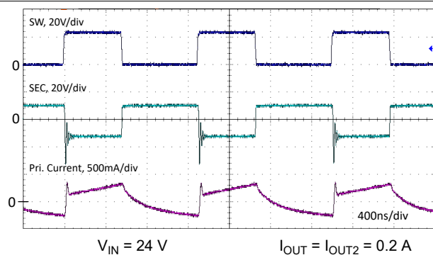
8-12. Typical Switching Waveforms
