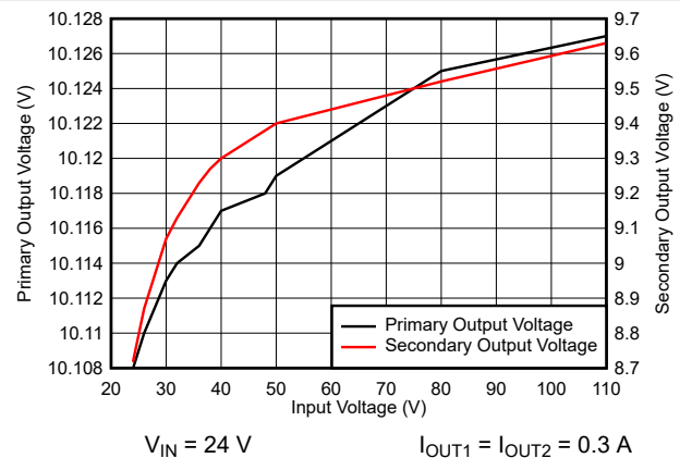
図 8-5. Line Regulation
