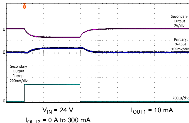
8-9. Load Transient on Secondary Output
