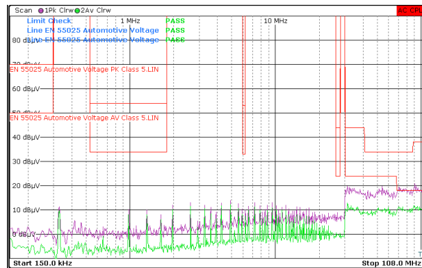
Figure 8-37. LM5169PDDAR Conducted EMI (Positive Rail)
