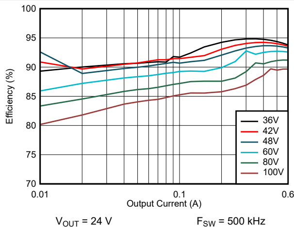
図 8-17. Efficiency: V_{OUT} = 24\text{ V}
