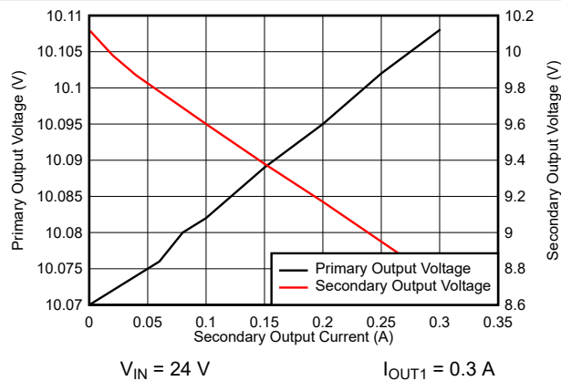
図 8-4. Load Regulation vs Secondary Load Current
