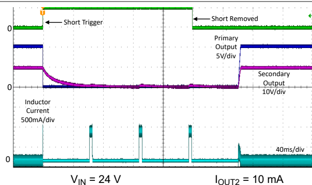
8-10. Short Circuit on Primary Output
