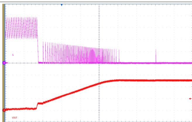
図 62. Short-Circuit Recovery
