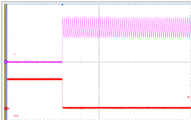
図 61. Short-Circuit Entry
