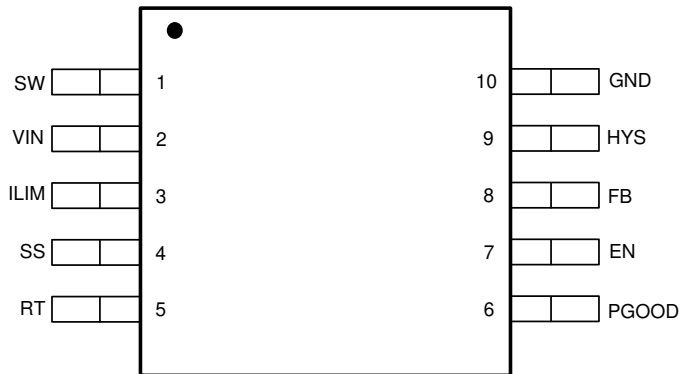
LM5165 Adjustable Output Version
