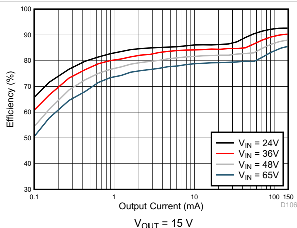
8-30. Efficiency
