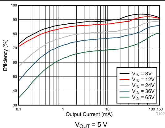
8-2. Efficiency
