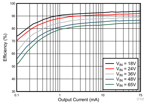
FIG 6-3. Converter Efficiency: 3.3 V, 50 mA, PFM
