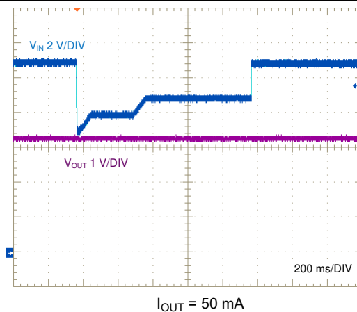
8-20. Input Voltage Transient (Automotive Cold Crank Profile)
