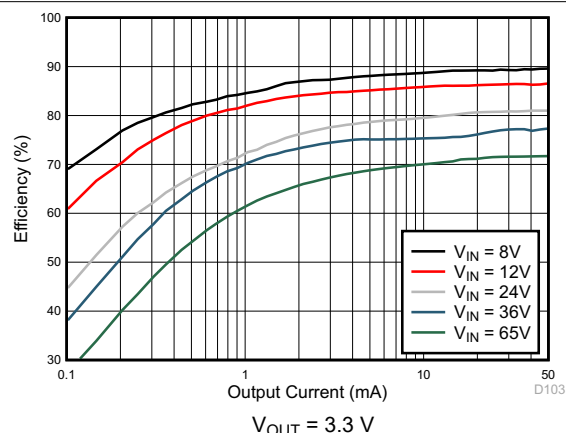
8-15. Efficiency
