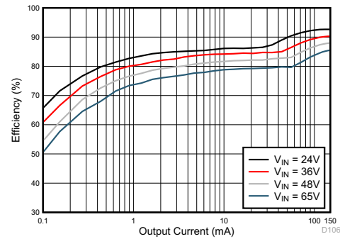
FIG 6-4. Converter Efficiency: 3.3 V, 150 mA, COT
