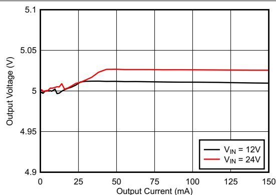
8-3. Load Regulation
