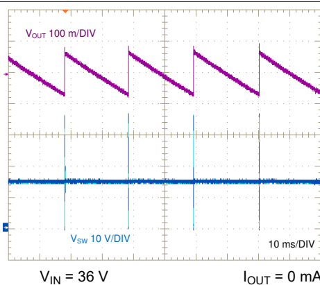
8-33. SW Node and Output Ripple Voltage, No Load
