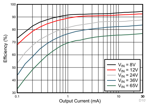
FIG 6-1. Converter Efficiency: 5 V, 25 mA, PFM
