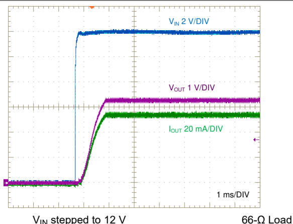
8-17. Start-Up, Full Load
