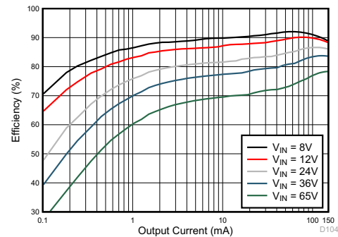
FIG 6-2. Converter Efficiency: 5 V, 150 mA, COT
