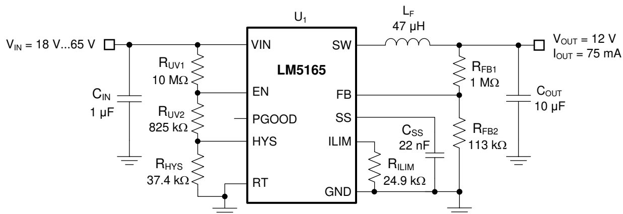
8-21. Schematic for Design 3 With V_{IN(nom)} = 24\text{ V} , V_{OUT} = 12\text{ V} , I_{OUT(max)} = 75\text{ mA} , F_{SW(nom)} = 500\text{ kHz}
