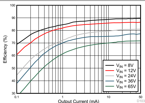
Figure 6-1. Converter Efficiency: 5 V, 25 mA, PFM
