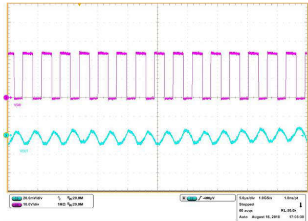
図 7-15. Full-Load Switching
