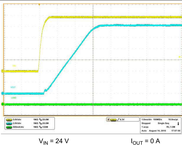
7-6. No-Load Start-up with VIN
