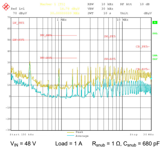
図 7-16. CISPR 25 Class 5 Conducted Emissions Plot, 150 kHz to 30 MHz
