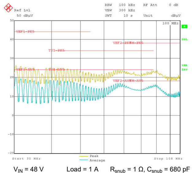
図 7-17. CISPR 25 Class 5 Conducted Emissions Plot, 30 MHz to 108 MHz
