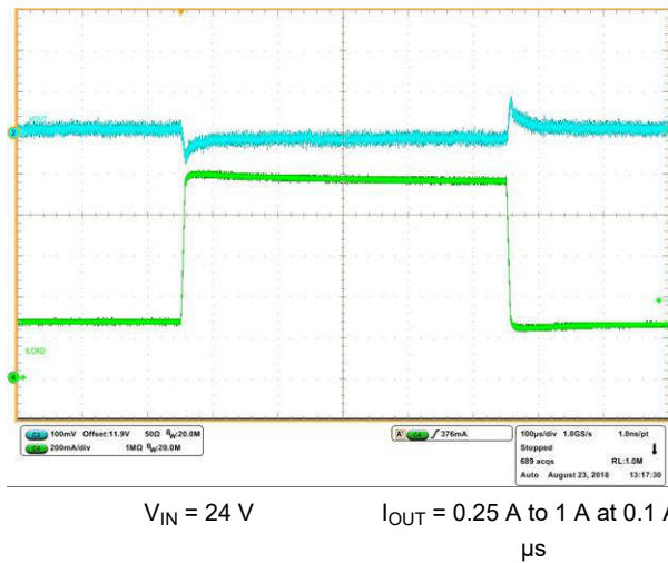
7-5. Load Step Response
