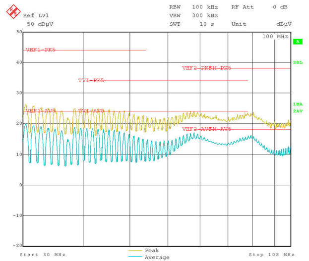
図 7-15. Full-Load Switching
