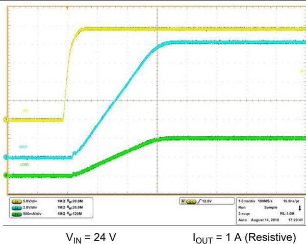
7-7. Full-Load Start-up with VIN
