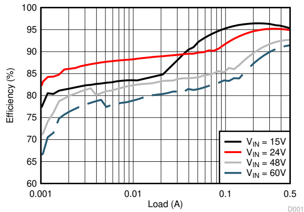
FIG 5-1. Conversion Efficiency (Log Scale)
