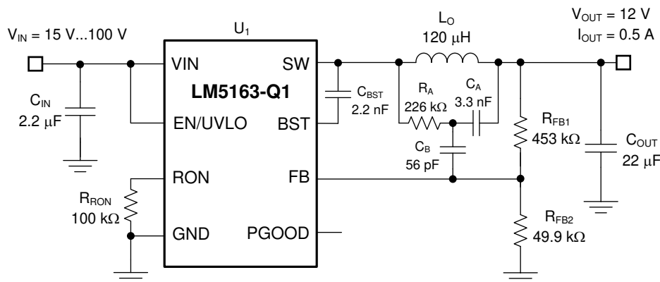
図 7-1. Typical Application V_{IN(nom)} = 48 \text{ V} , V_{OUT} = 12 \text{ V} , I_{OUT(max)} = 0.5 \text{ A} , F_{SW(nom)} = 300 \text{ kHz}
