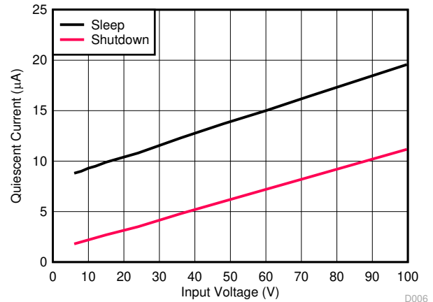
FIG 5-4. V_{IN} Shutdown and Sleep Supply Current versus Input Voltage
