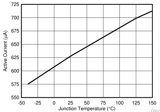
FIG 5-5. V_{IN} Active Current versus Temperature
