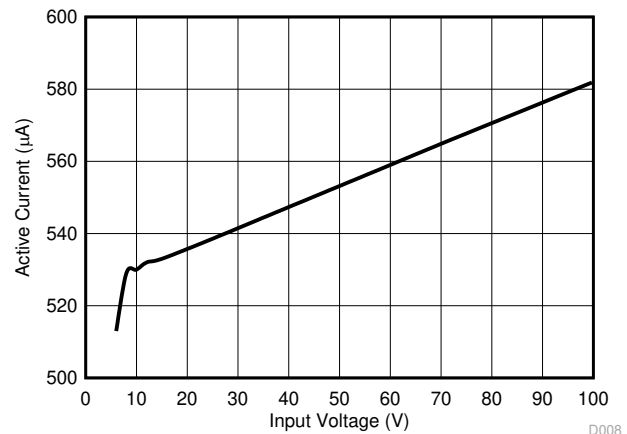
FIG 5-6. V_{IN} Active Current versus Input Voltage
