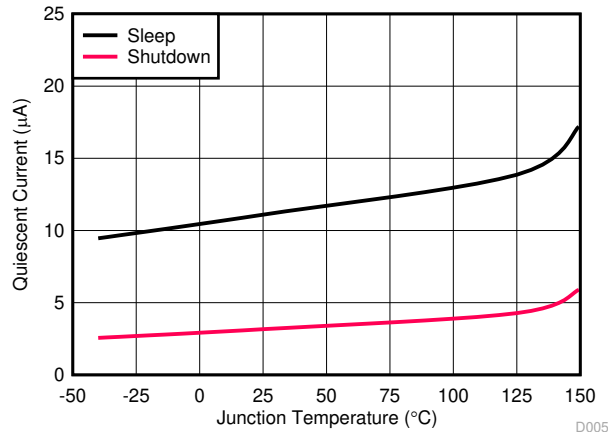
FIG 5-3. V_{IN} Shutdown and Sleep Supply Current versus Temperature
