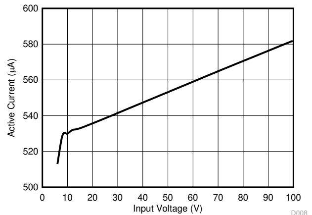
図 5-6. V_{\text{IN}} Active Current versus Input Voltage
