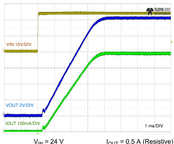
7-7. Full-Load Start-up with VIN
