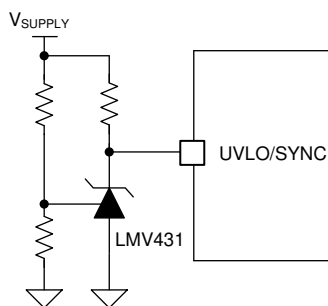
9-16. Inverted UVLO
