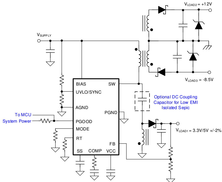
FIG 10-9. Primary-Side Regulated Multiple-Output Isolated Flyback/Isolated SEPIC
