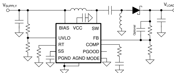
FIG 10-4. Typical SEPIC Application
