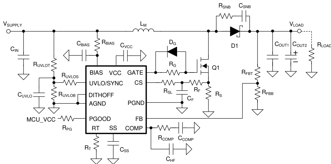
FIG 10-1. Typical Boost Converter Circuit With Optional Components
