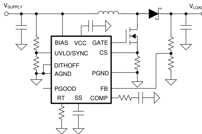
FIG 10-3. Typical Boost Application
