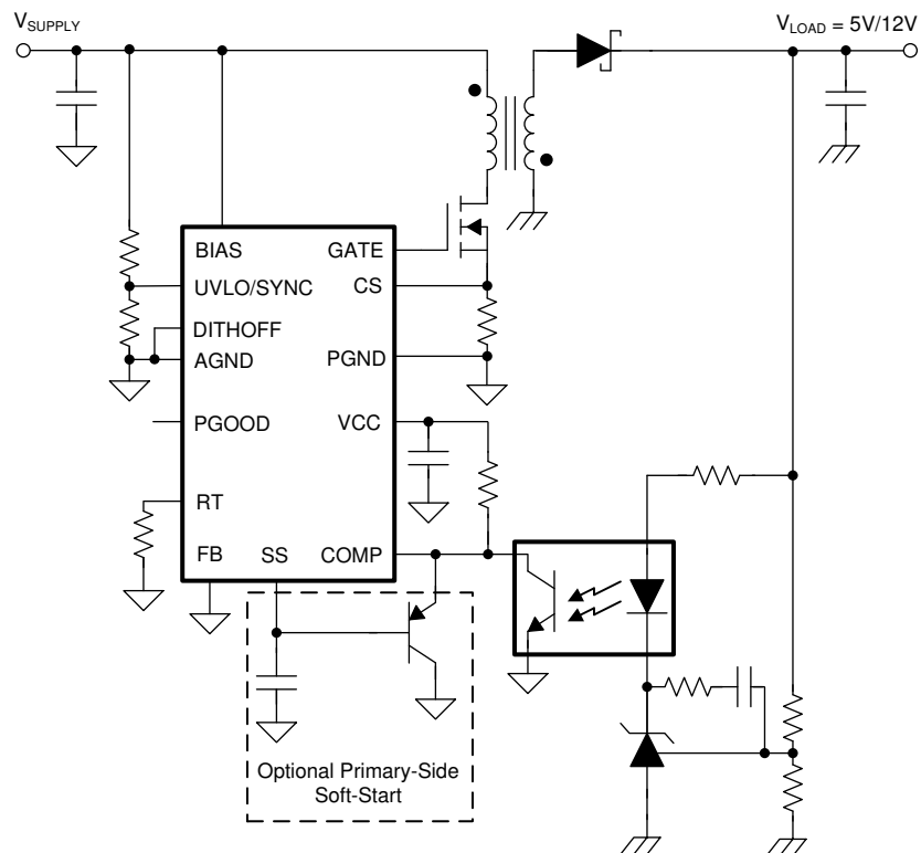
FIG 10-10. Secondary-Side Regulated Isolated Flyback
