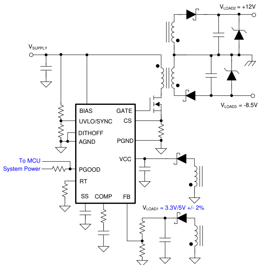
FIG 10-11. Primary-Side Regulated Multiple-Output Isolated Flyback
