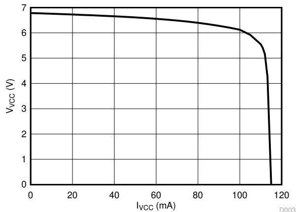
8-3. V_{VCC} vs I_{VC}
