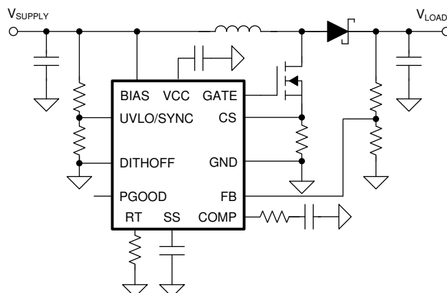
10-3. Typical Boost Application
