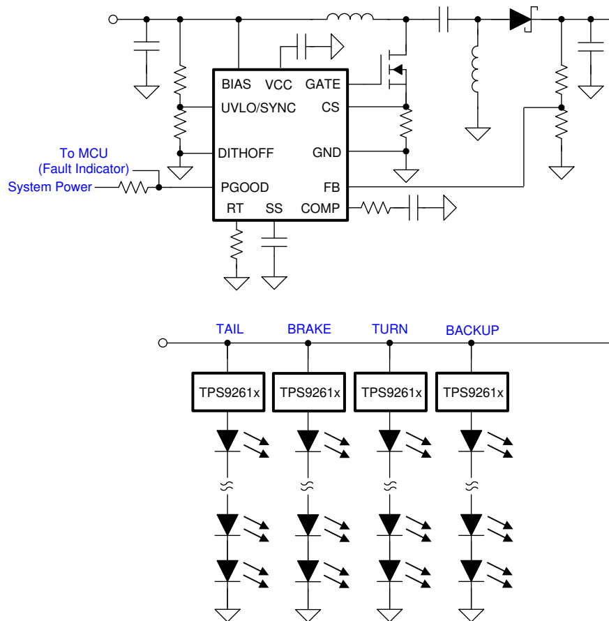
FIG 10-14. Dual-Stage Automotive Rear-Lights LED Driver
