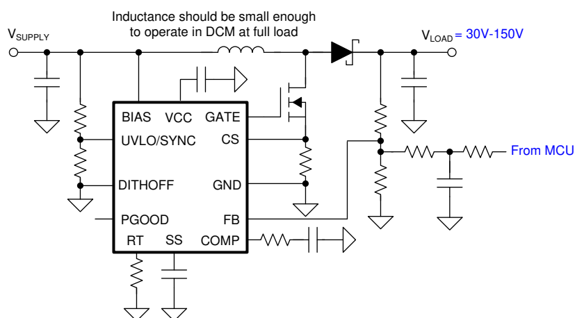
FIG 10-7. LIDAR Bias Supply 1
