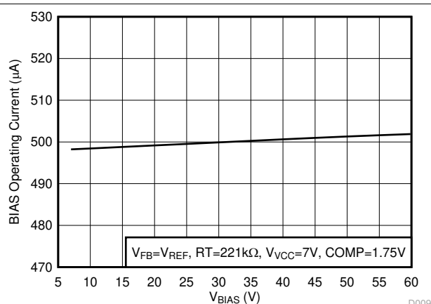
8-9. I_{OPERATING(BIAS)} Including RT Current vs V_{BIAS}
