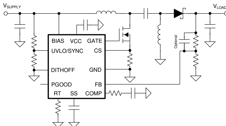
FIG 10-6. Typical SEPIC Application
