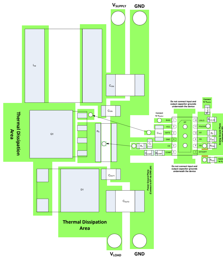
12-1. PCB Layout Example 1
