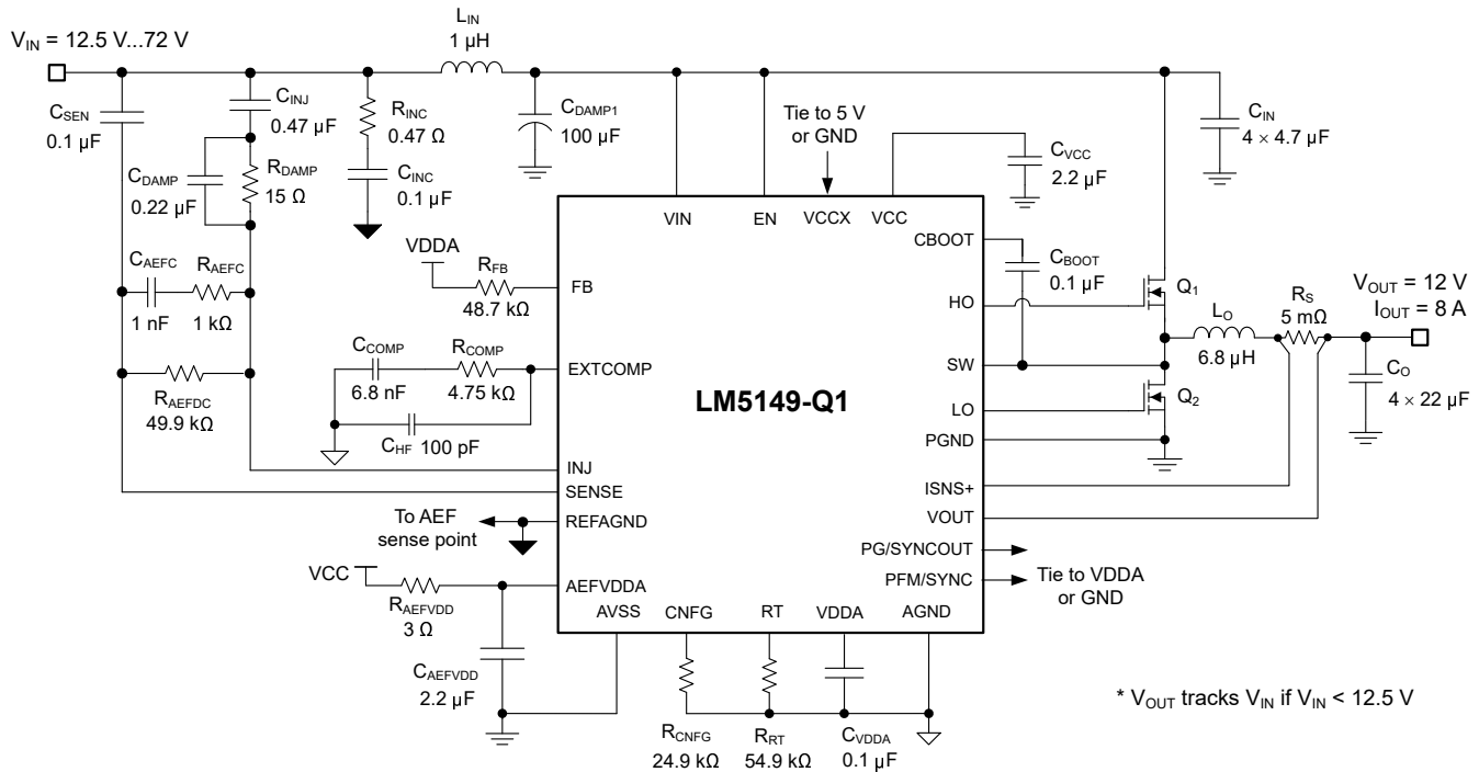
9-18. Application Circuit 2 With LM5149-Q1 Buck Regulator at 400 kHz
