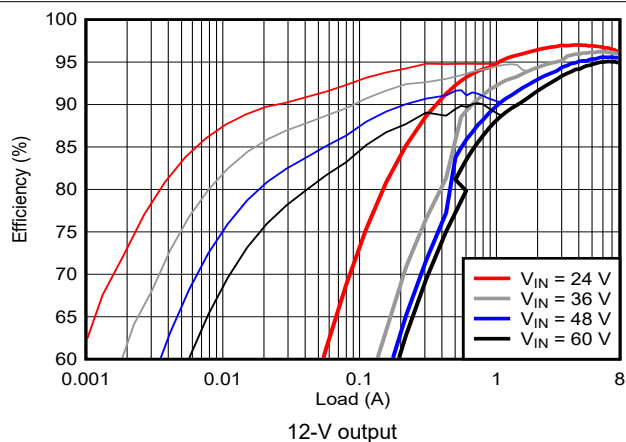
9-20. Efficiency vs. I_{OUT} , Log Scale
