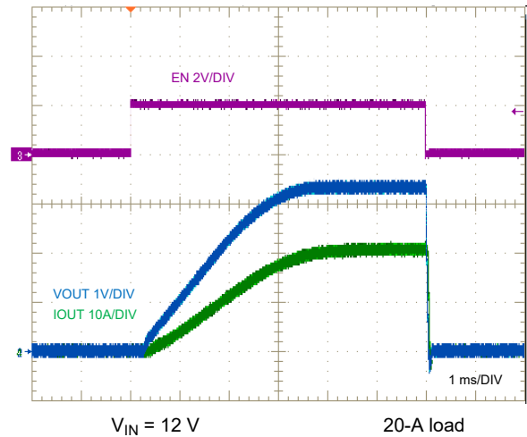
9-44. ENABLE ON and OFF Characteristic
