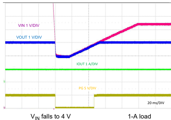
9-35. Line Transient Response to V_{IN} = 4 V
