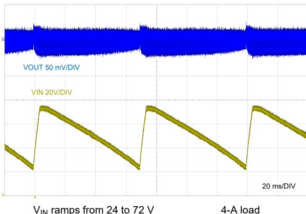
9-24. Line Transient Response to V_{IN} = 72 V
