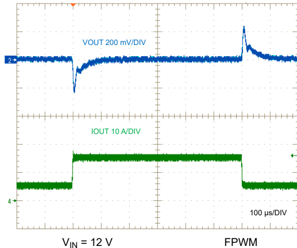
9-45. Load Transient, 5 A to 15 A
