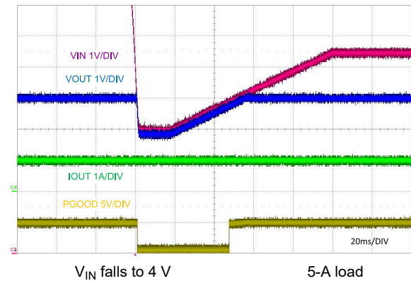
9-11. Line Transient Response to V_{IN} = 4 V
