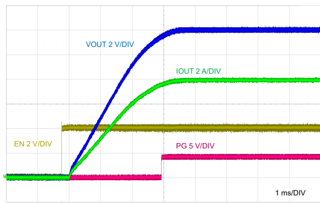
図 8-24. EN Start-Up Characteristic
