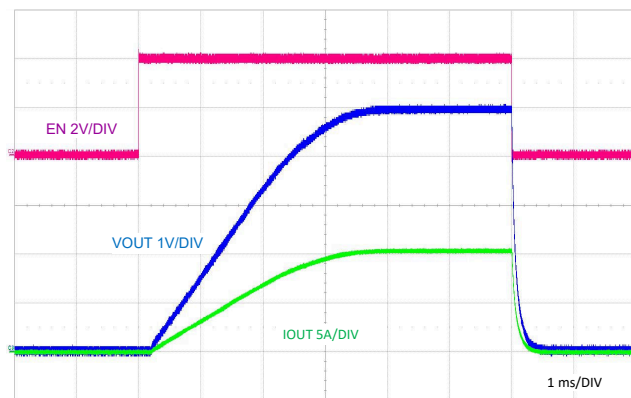
図 8-36. ENABLE ON and OFF Characteristic
