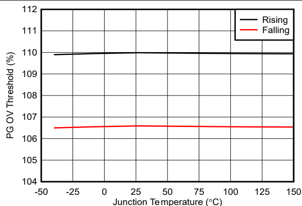
図 6-9. PG OV Thresholds vs Temperature
