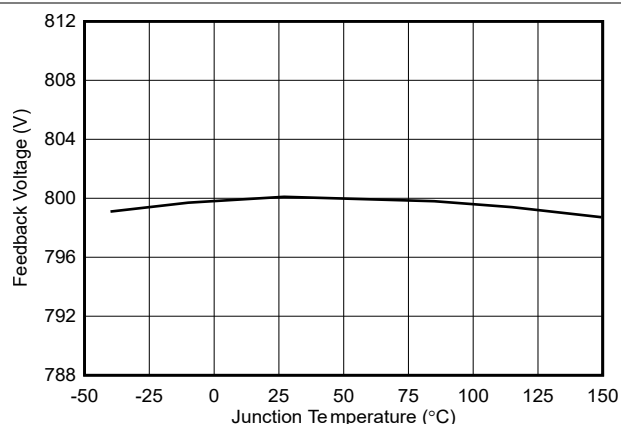
図 6-8. Feedback Voltage vs Temperature
