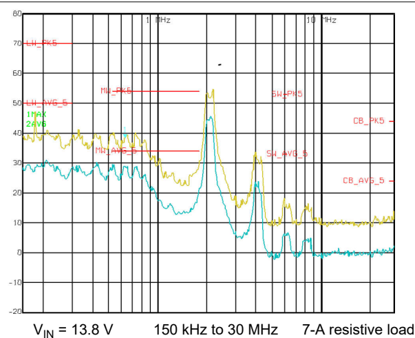
図 8-16. CISPR 25 Class 5 Conducted EMI
