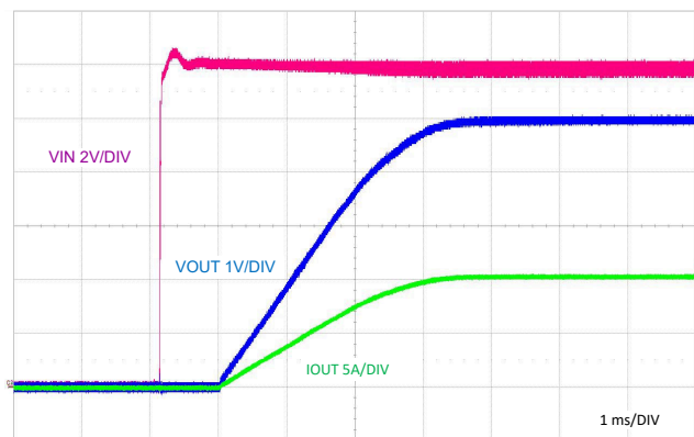
図 8-35. Start-Up Characteristic
