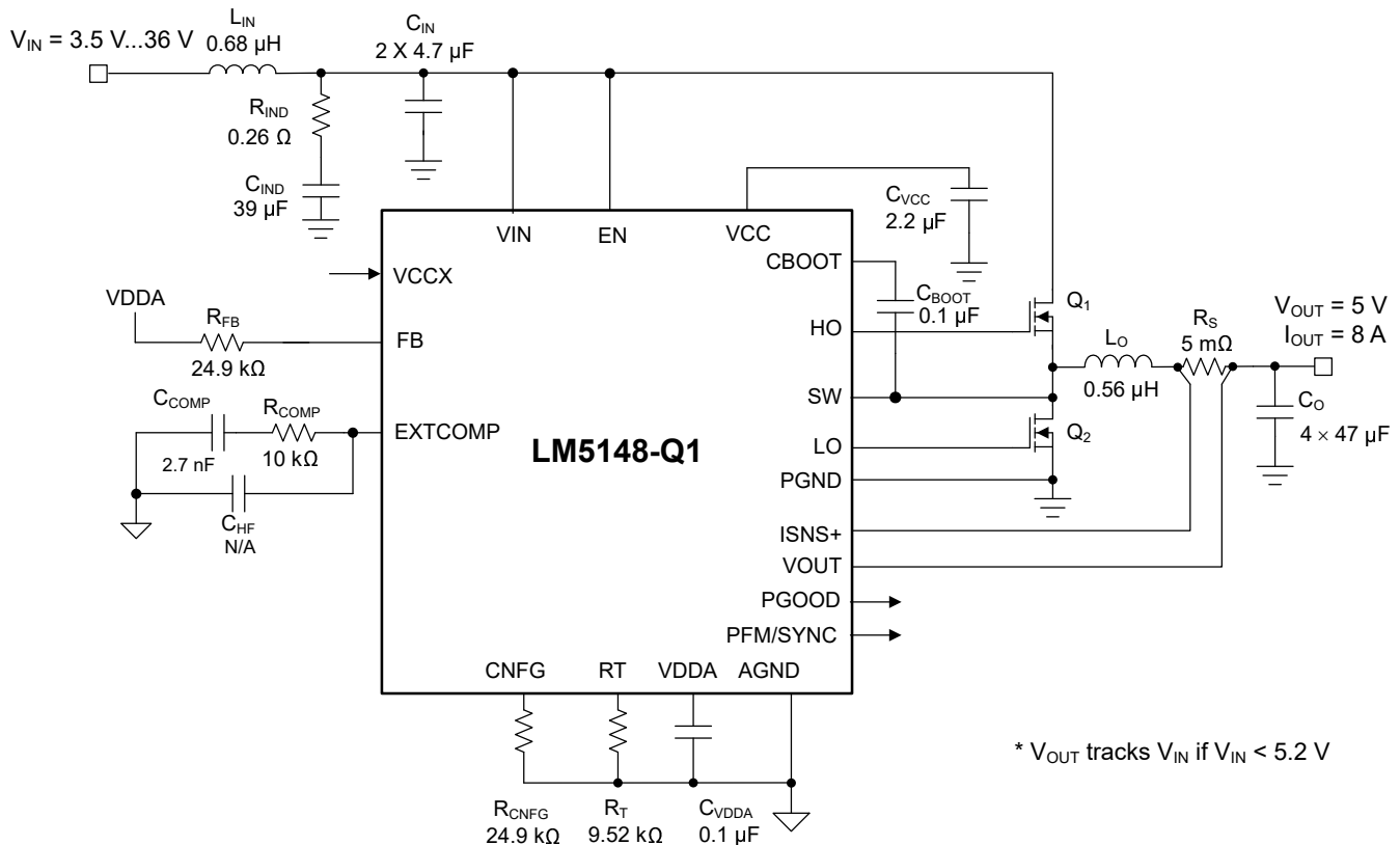
8-4. Application Circuit 1 With LM5148-Q1 Buck Regulator Switching at 2.1 MHz
