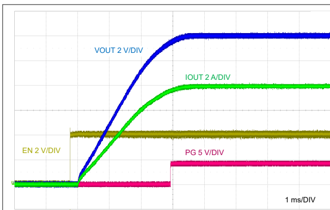
図 9-24. EN Start-Up Characteristic
