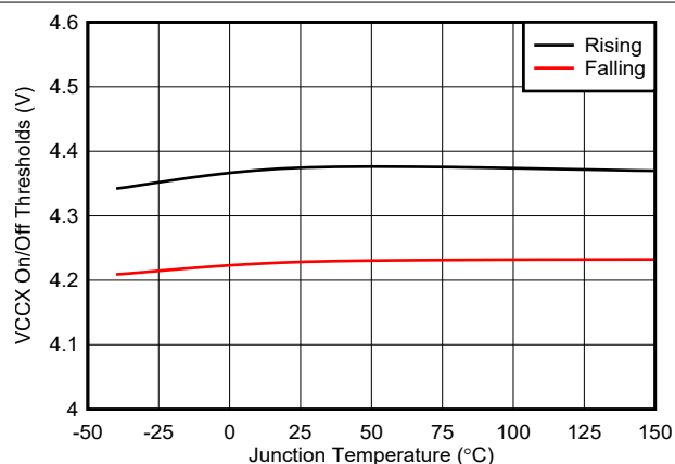
FIG 7-16. VCCX On, Off Thresholds vs Temperature
