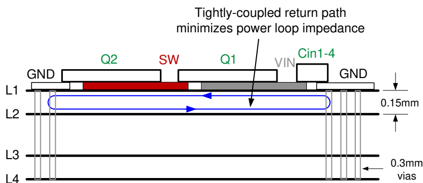
FIG 9-49. PCB Stack-up Diagram With Low L1-L2 Intra-layer Spacing 1
