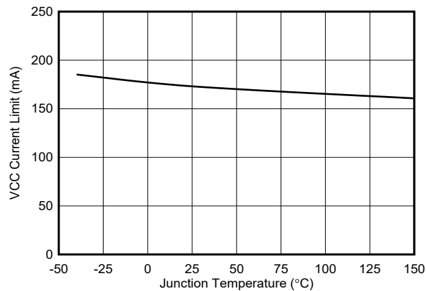
FIG 7-13. VCC Current Limit vs Temperature
