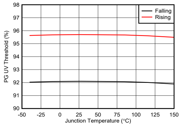
图 7-10. PG UV Thresholds vs Temperature
