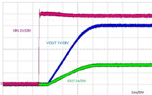
图 9-11. Start-Up Characteristic
