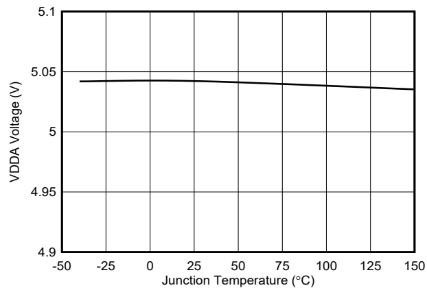
FIG 7-14. VDDA Regulation Voltage vs Temperature
