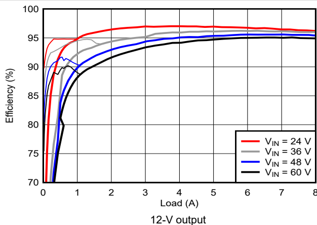
图 9-18. Efficiency vs. I_{OUT}
