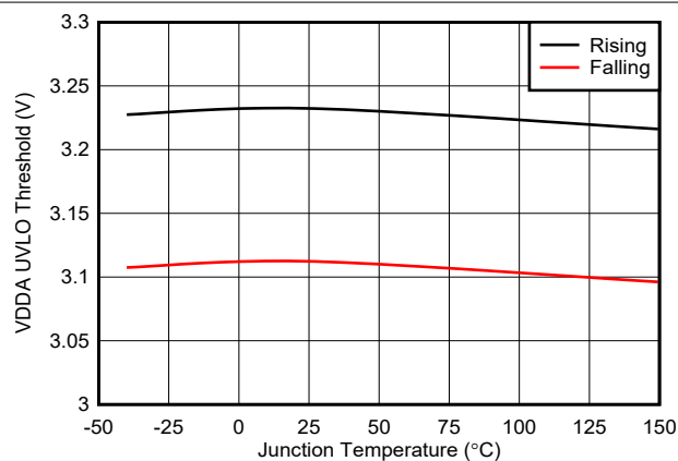
FIG 7-15. VDDA UVLO Thresholds vs Temperature
