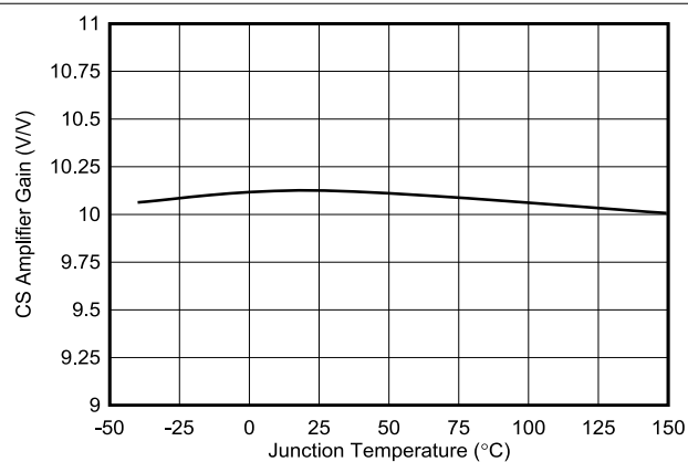
FIG 7-18. Current Sense (CS) Amplifier Gain vs Temperature
