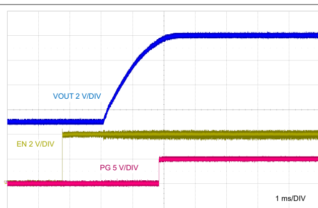
図 9-25. EN Start-Up Pre-bias Characteristic
