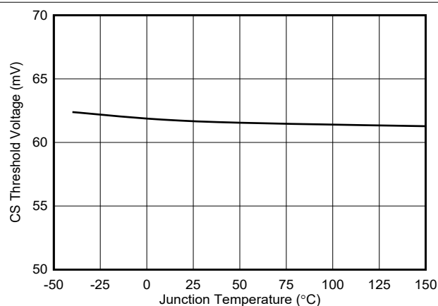
FIG 7-17. Current Sense (CS) Threshold vs Temperature
