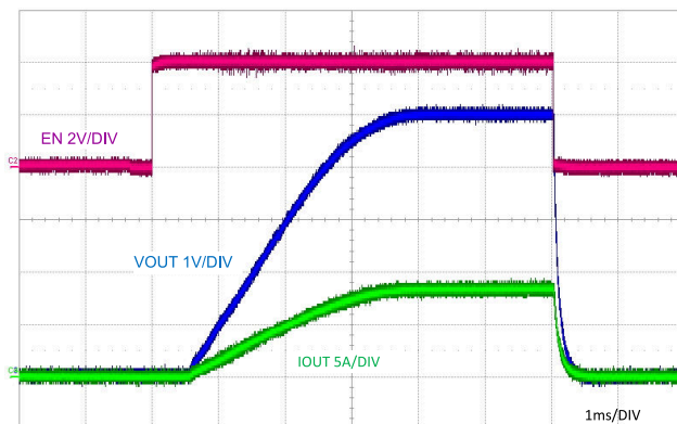
图 9-12. ENABLE ON and OFF Characteristic
