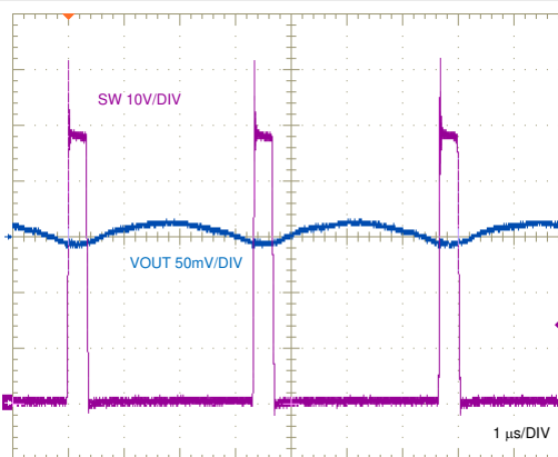
9-15. SW Node and Output Ripple Voltages
