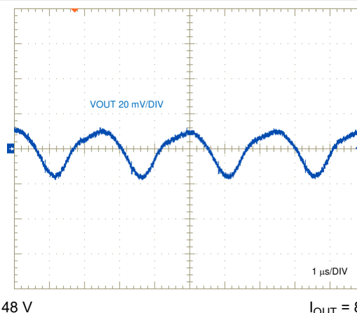
图 9-26. Output Voltage Ripple
