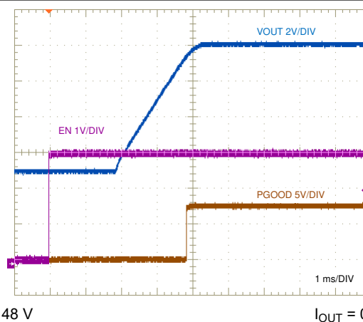
图 9-28. Pre-Biased Start-Up
