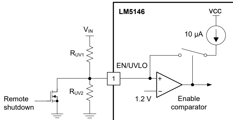
FIG 8-3. Programmable Input Voltage UVLO Turn-on and Turn-off
