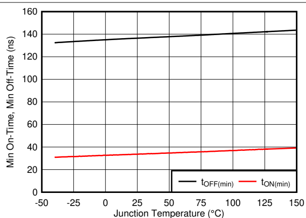
图 7-4. t_{ON(min)} and t_{OFF(min)} vs Junction Temperature
