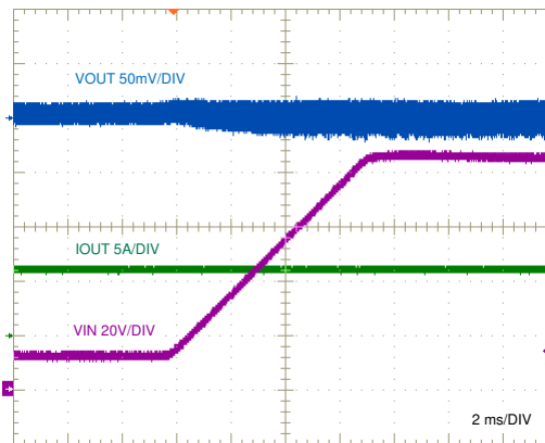
FIG 9-13. Line Transient Response, 12 V to 85 V
