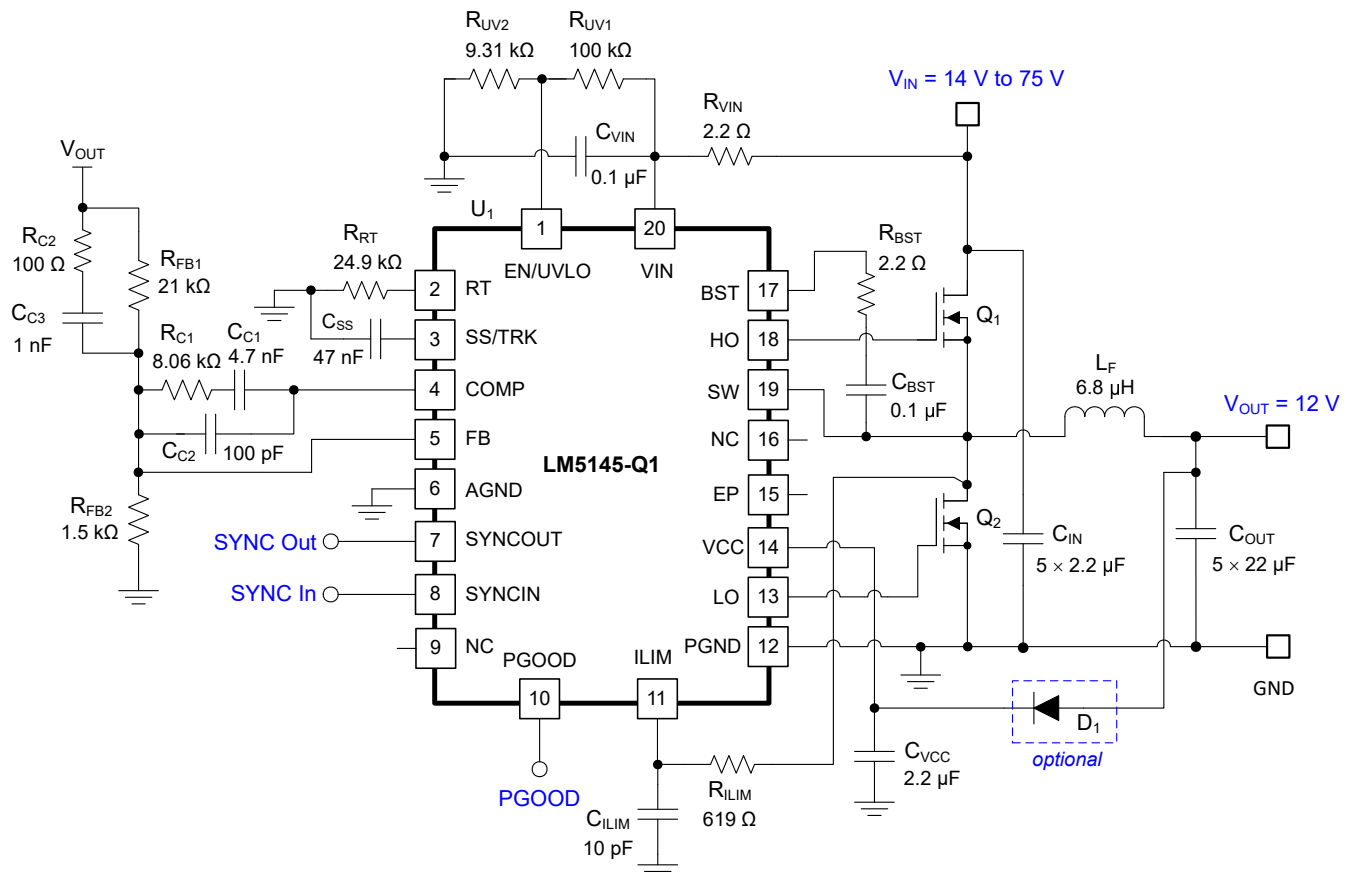
9-16. Application Circuit 2 With LM5145-Q1 48-V to 12-A Synchronous Buck Regulator at 400 kHz
