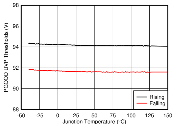
FIG 7-14. PGOOD UVP Thresholds vs Junction Temperature
