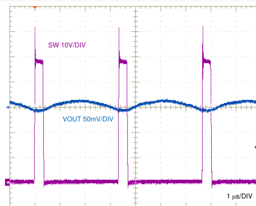
FIG 9-15. SW Node and Output Ripple Voltages
