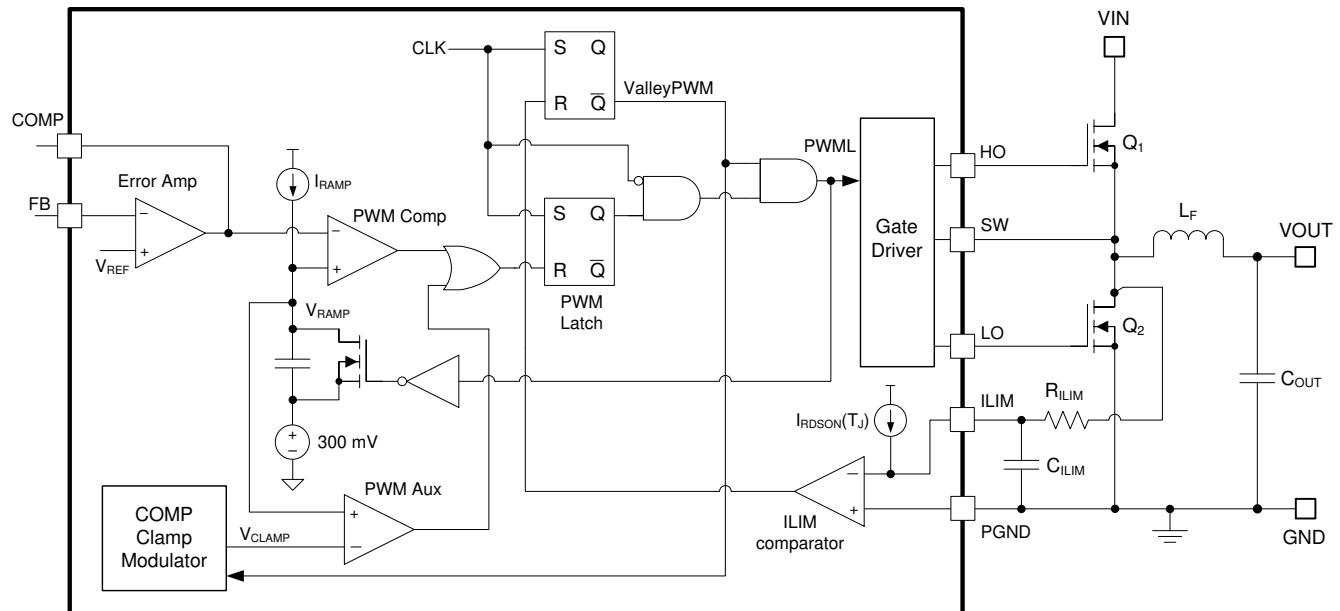
FIG 8-10. OCP Setpoint Defined by Current Source I_{RDSON} and Resistor R_{ILIM} in R_{DS-ON} Mode
