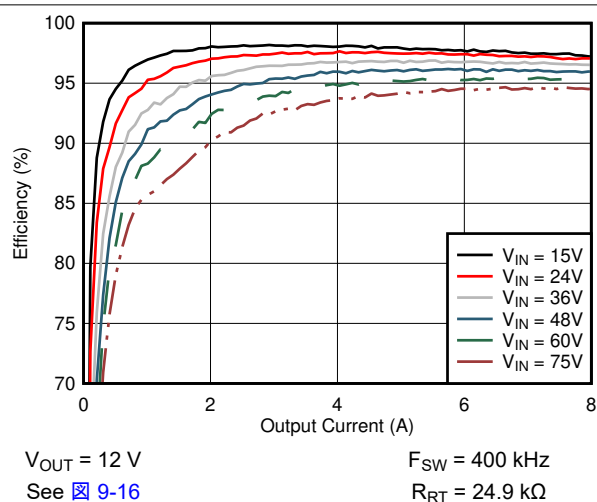
图 7-2. Efficiency vs Load, CCM
