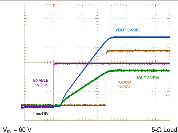
9-38. ENABLE ON, 5-A Resistive Load
