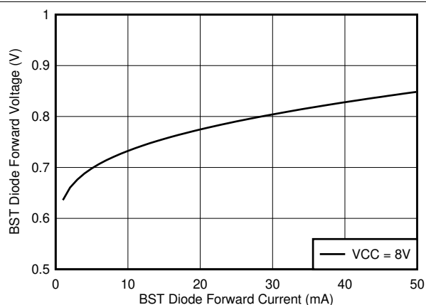
FIG 7-23. BST Diode Forward Voltage vs Current
