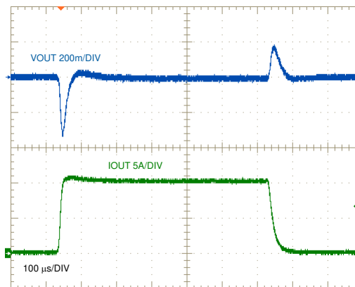
9-28. Load Transient Response, 0 A to 10 A to 0 A
