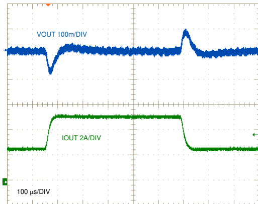
FIG 9-40. Load Transient Response, 2.5 A to 5 A to 2.5 A
