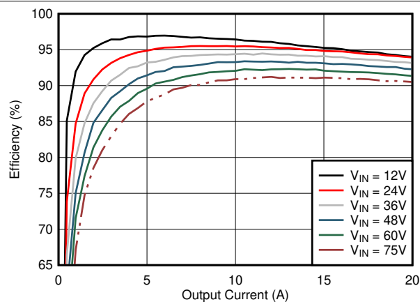
FIG 9-6. Efficiency and Power Loss vs I_{OUT} and V_{IN}
