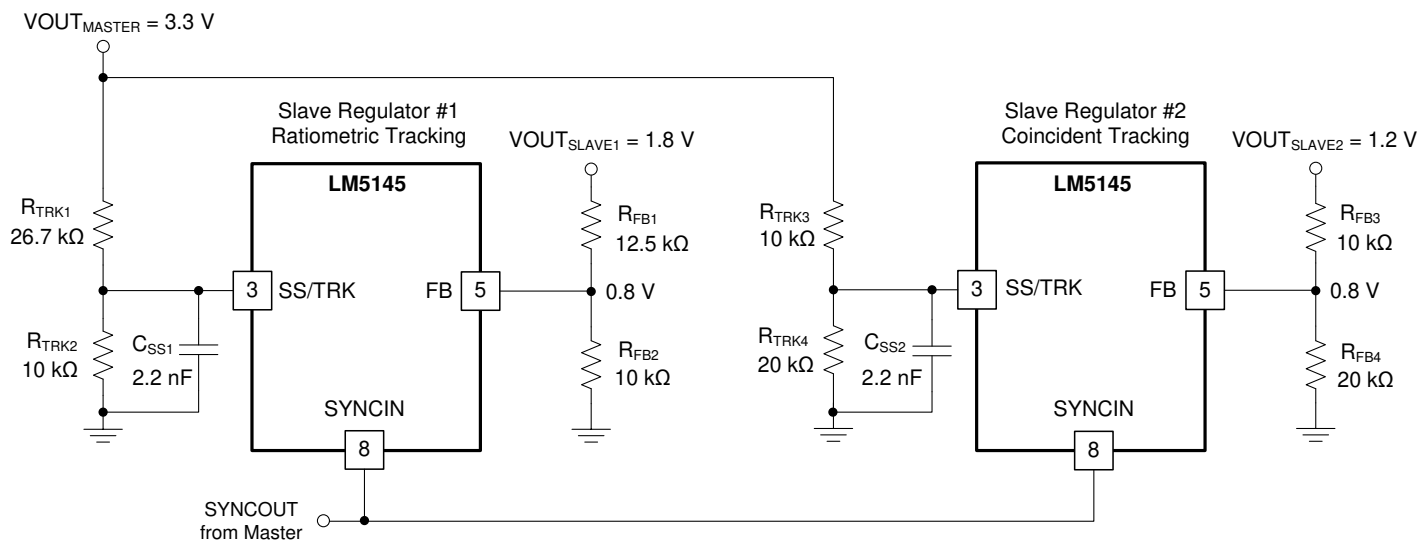
FIG 8-7. Tracking Implementation With Master, Ratiometric Slave, and Coincident Slave Rails
