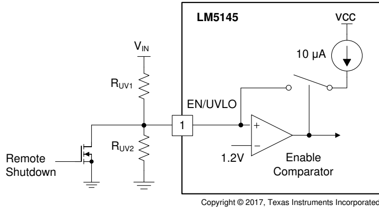
FIG 8-3. Programmable Input Voltage UVLO Turnon and Turnoff
