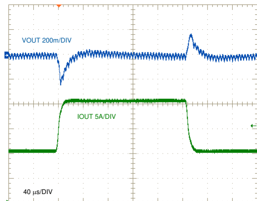
FIG 9-12. Load Transient Response, 10 A to 20 A to 10 A
