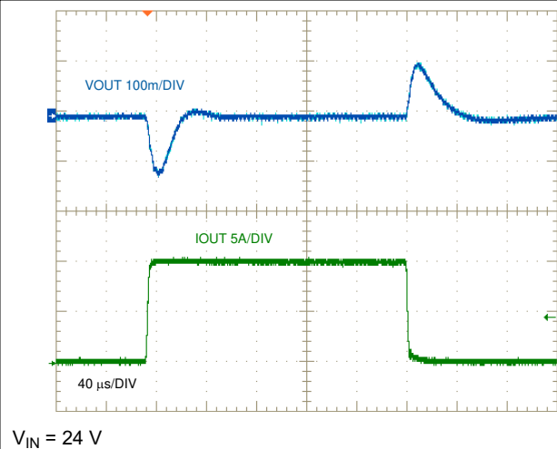
9-50. Load Transient Response, 0 A to 10 A to 0 A
