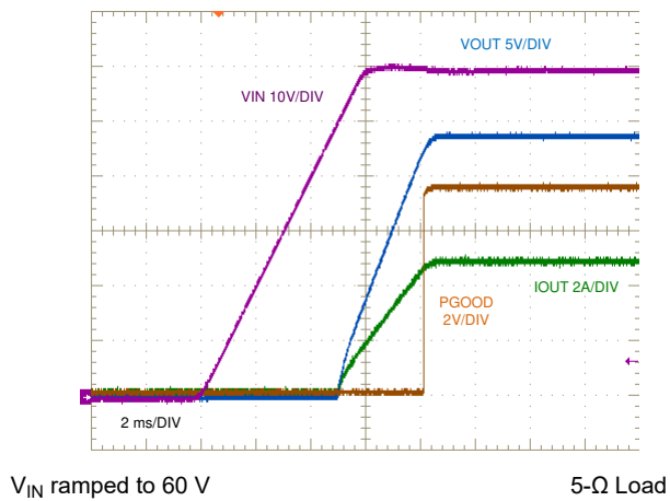
9-36. Start-Up, 5-A Resistive Load
