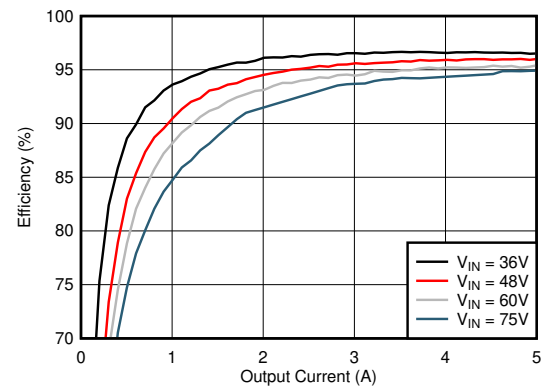
7-2. Efficiency vs Load, DCM
