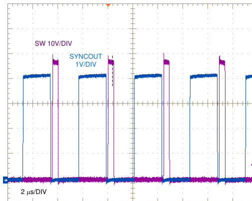
FIG 9-7. SYNCOUT and SW Node Voltages
