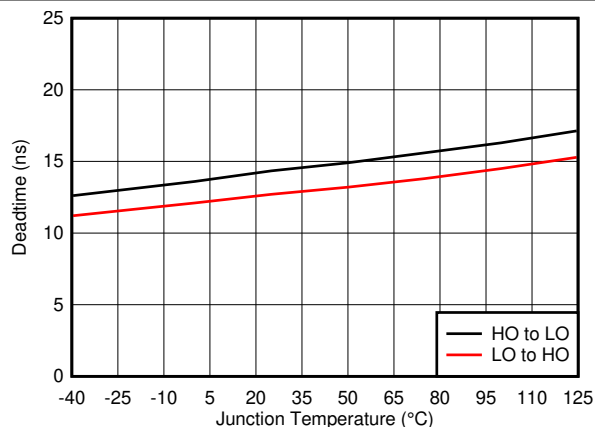
7-14. Deadtime vs Junction Temperature
