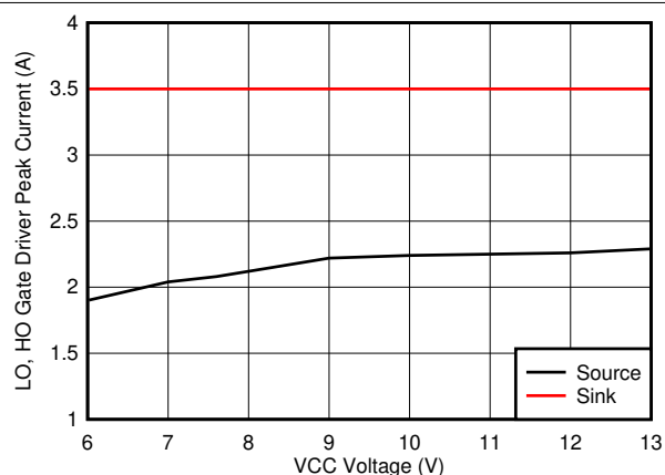
FIG 7-24. Gate Driver Peak Current vs VCC Voltage
