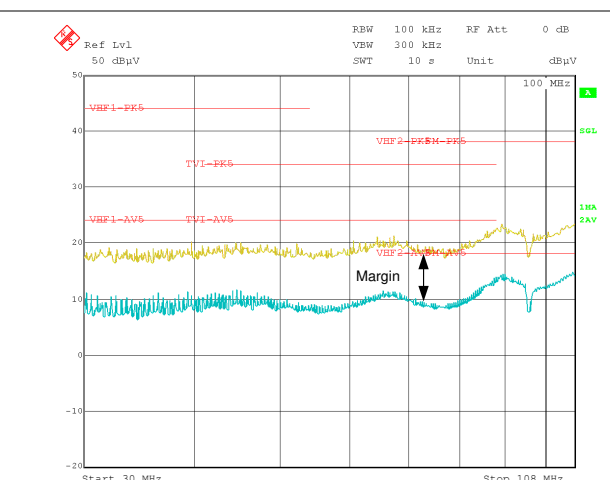
9-19. CISPR 25 Class 5 Conducted EMI, 30 MHz to 108 MHz
