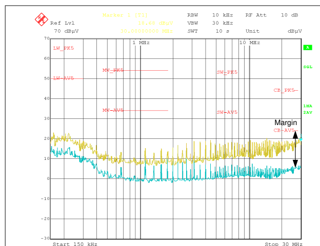
9-18. CISPR 25 Class 5 Conducted EMI, 150 kHz to 30 MHz
