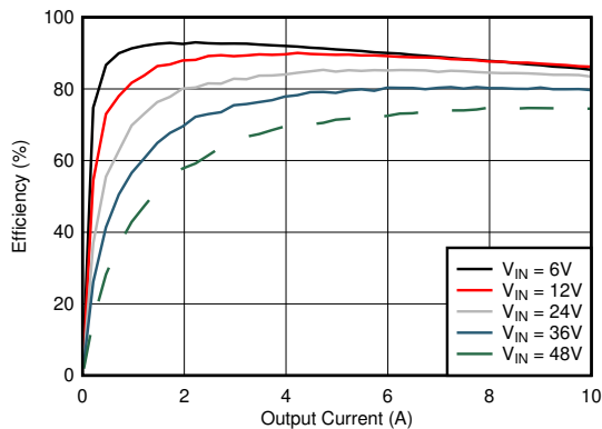
7-3. Efficiency vs Load, CCM
