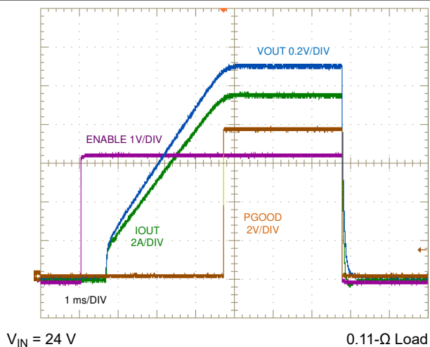
9-49. ENABLE ON and OFF, 10-A Resistive Load
