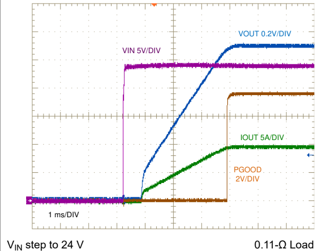
9-48. Start-Up, 10-A Resistive Load
