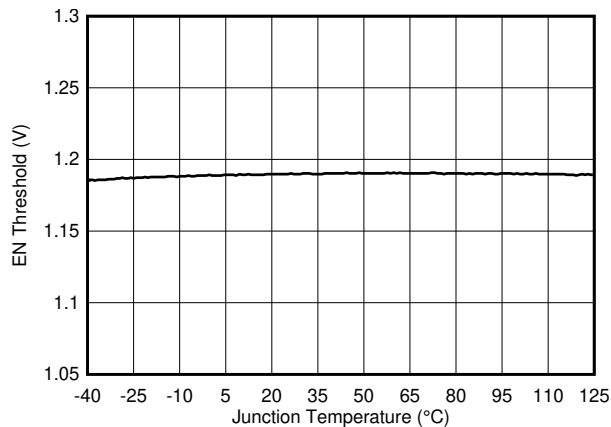
FIG 7-19. EN/UVLO Threshold vs Junction Temperature
