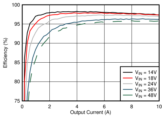
7-1. Efficiency vs Load, CCM
