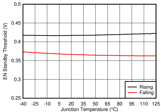
FIG 7-20. EN Standby Thresholds vs Junction Temperature
