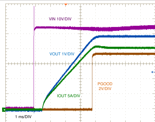
FIG 9-8. Start-Up, 20-A Resistive Load
