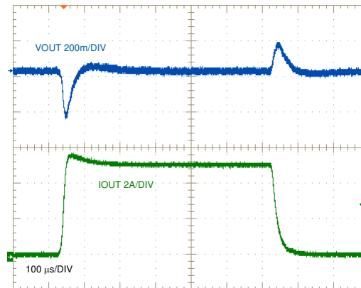
FIG 9-41. Load Transient Response, 0 A to 5 A to 0 A
