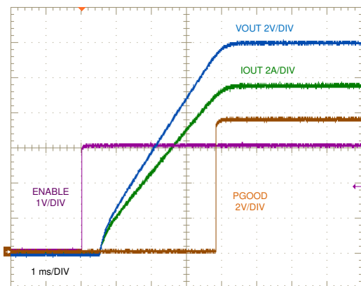
9-23. Start-Up, 10-A Resistive Load
