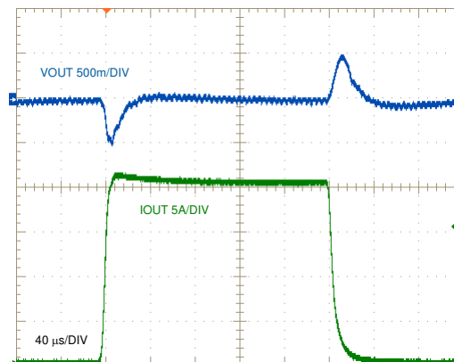
FIG 9-13. Load Transient Response, 0 A to 20 A to 0 A
