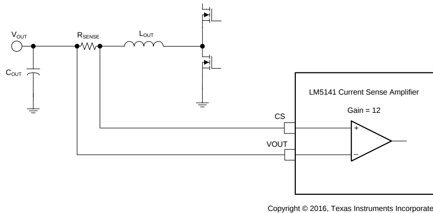
Figure 24. Current Sense
