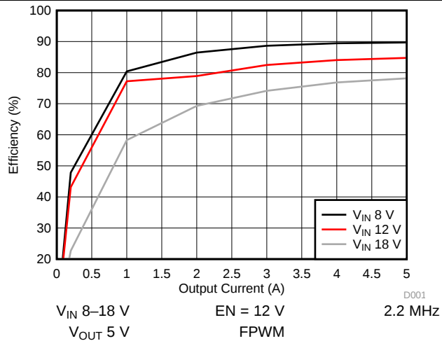
Figure 1. Efficiency vs I_{OUT}
