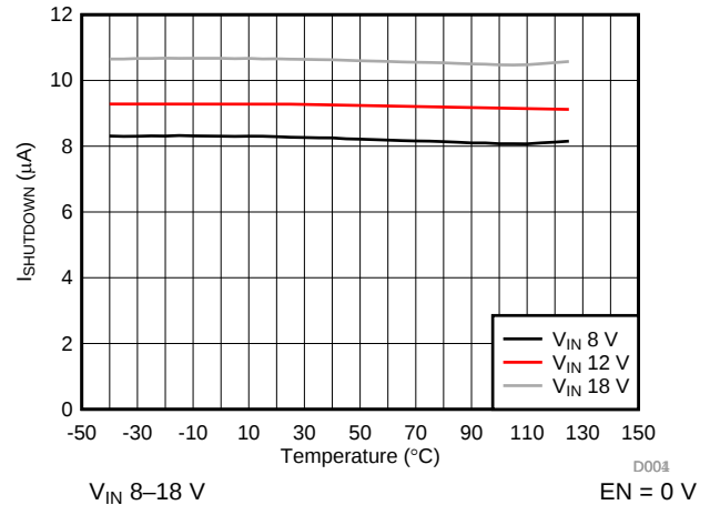
Figure 4. I_{SHUTDOWN} vs Temperature
