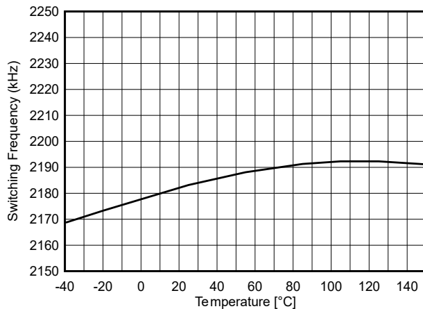
図 5-3. Switching Frequency (2200kHz, RT = 14kΩ) vs Temperature
