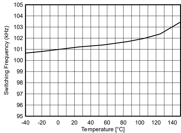
図 5-2. Switching Frequency (100kHz, RT = 316kΩ) vs Temperature
