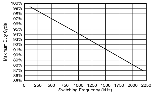
Figure 5-12. Maximum Duty Cycle vs Switching Frequency
