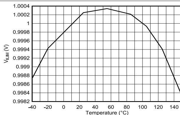
Figure 5-18. Average Current Limit Regulation Voltage vs Temperature
