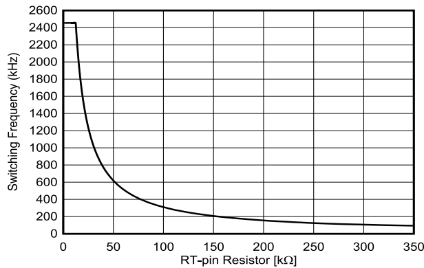
図 5-1. Switching Frequency Versus RT Resistance
