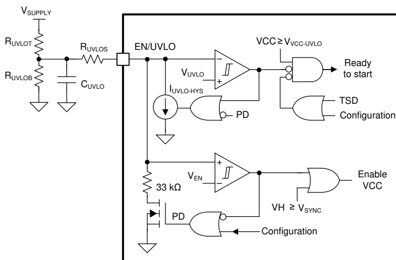
FIG 7-1. EN/UVLO Circuit
