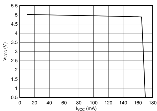
Figure 6-9. V CC vs I CC
