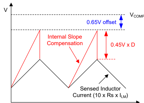
FIG 7-14. PWM Comparator Input
