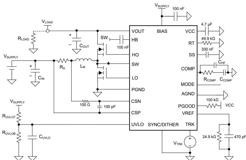
図 8-1. Typical Synchronous Boost Converter with Optional Components
