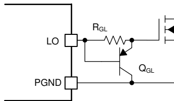
FIG 7-19. Slew Rate Control
