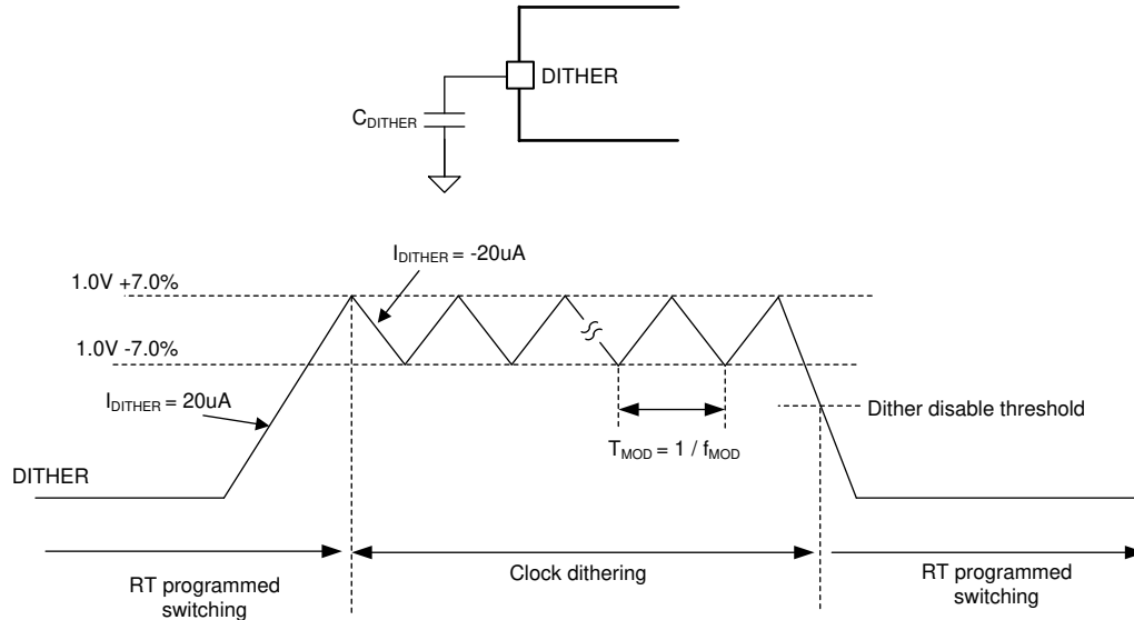
FIG 7-10. Switching Frequency Dithering
