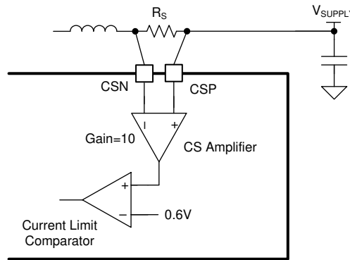
FIG 7-15. Current Limit Comparator
