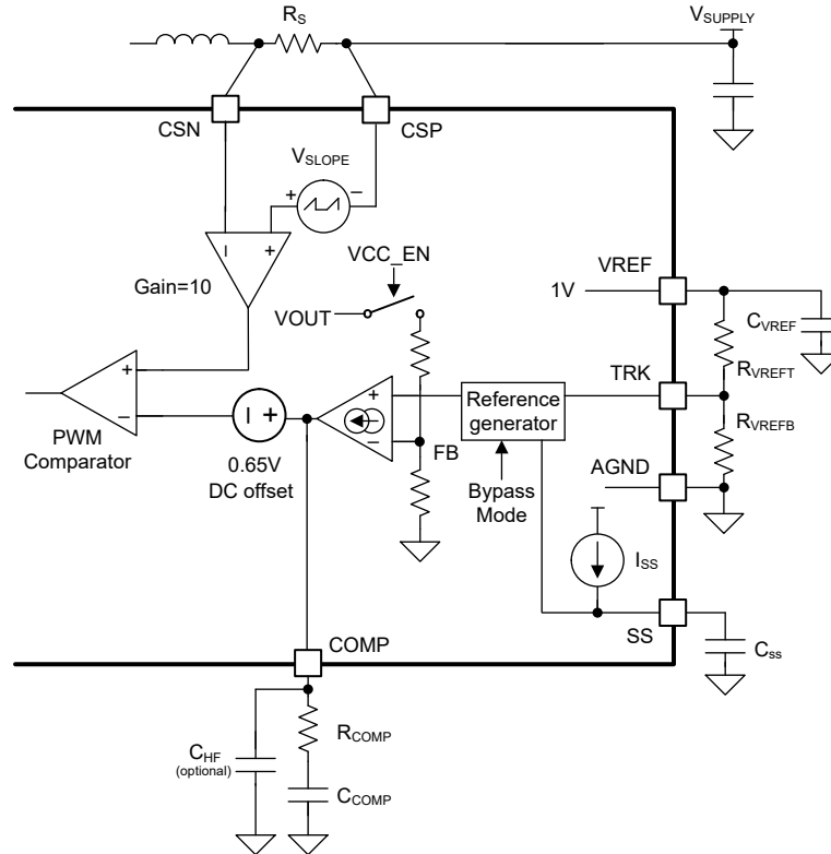
FIG 7-13. Error Amplifier, Current Sense Amplifier and PWM
