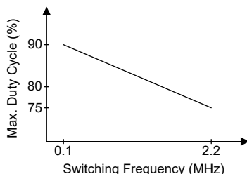
FIG 7-17. Switching Frequency vs max. Duty Cycle
