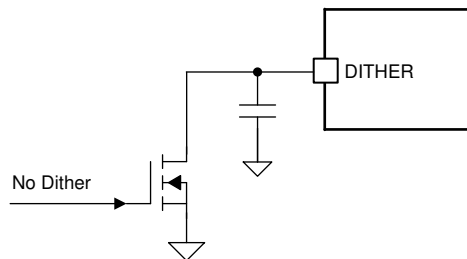
FIG 7-11. Dynamic Dither On/Off Example
