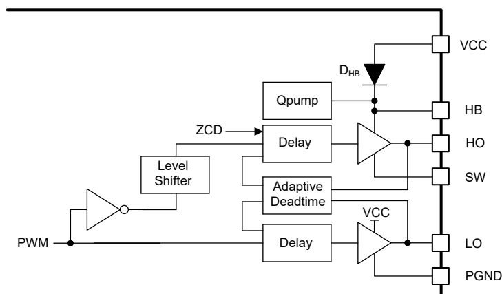
FIG 7-18. Driver Structure with Internal Boot Diode
