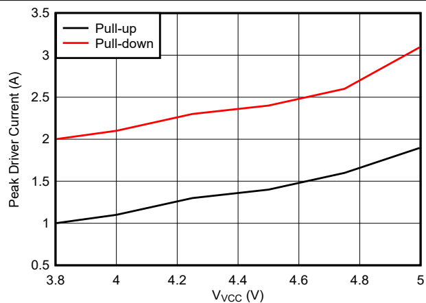
Figure 6-16. V CC vs Peak Driver Current
