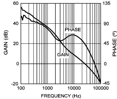
図 7-5. Overall Voltage Loop Gain and Phase
