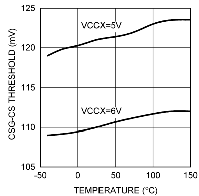
5-18. Current Limit Threshold vs Temperature
