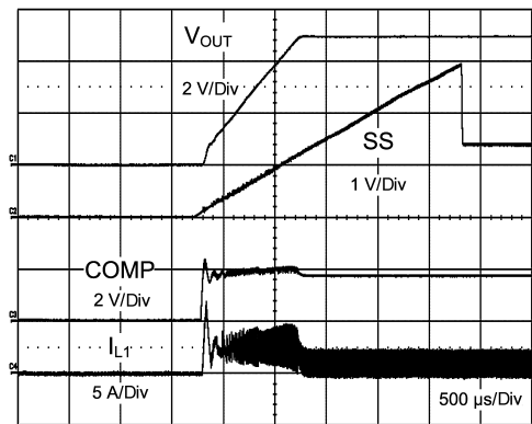
図 7-9. Short-Circuit Recovery Into Resistive Load With C7 = 1 μF and D2 Installed
