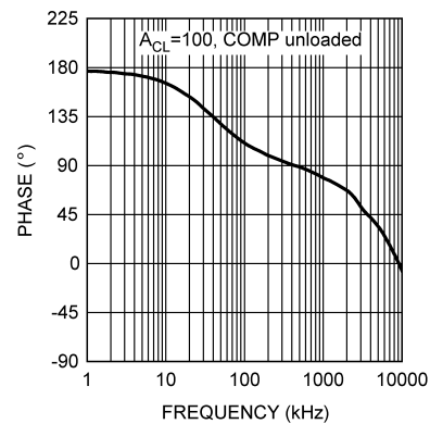
5-16. Error Amp Phase vs Frequency
