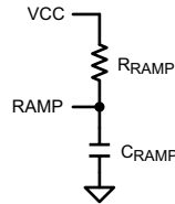
FIG 7-6. R_{RAMP} to VCC for V_{OUT} > 7.5 \text{ V}
