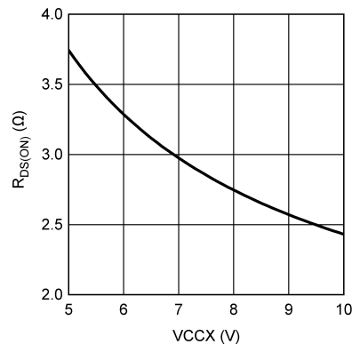
FIG 5-24. VCCX Switch R_{DS(ON)} vs VCCX
