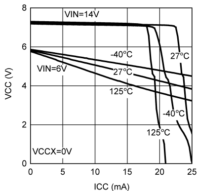
FIG 5-23. VCC vs ICC
