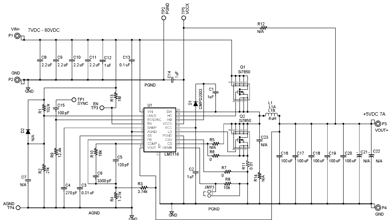
図 7-1. 5-V 7-A Typical Application Schematic
