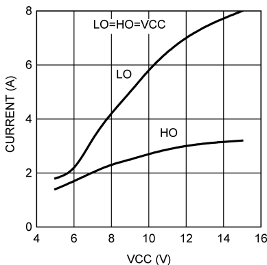
5-5. Driver Sink Current vs VCC
