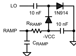
FIG 7-7. R_{RAMP} to -VCC for V_{OUT} < 7.5 \text{ V}
