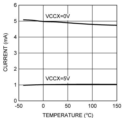
FIG 5-19. VIN Operating Current vs Temperature
