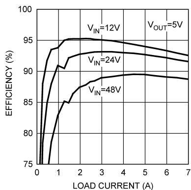
5-1. Typical Application Circuit Efficiency
