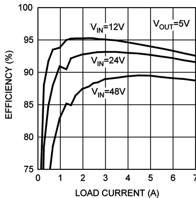
図 7-8. Efficiency With 6-μH Copper Inductor
