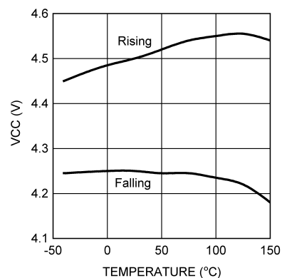
FIG 5-21. VCC UVLO vs Temperature
