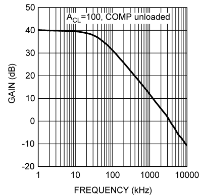
5-14. Error Amp Gain vs Frequency
