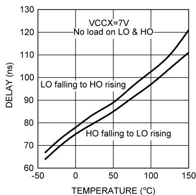
5-3. Driver Dead-time vs Temperature
