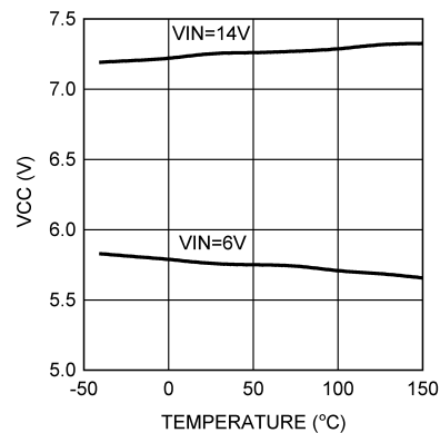
FIG 5-20. VCC vs Temperature
