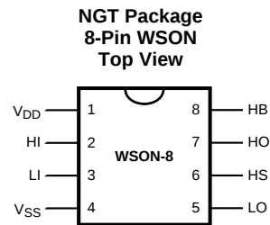
Pin Functions
