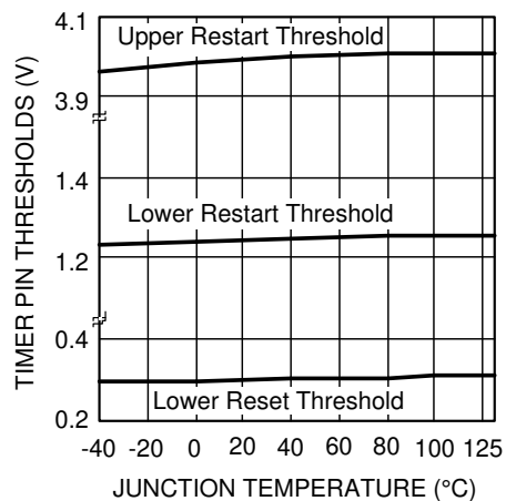
FIG 7-20. TIMER Pin Thresholds vs Temperature
