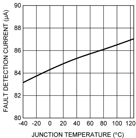
FIG 7-21. TIMER Pin Fault Detection Current vs Temperature
