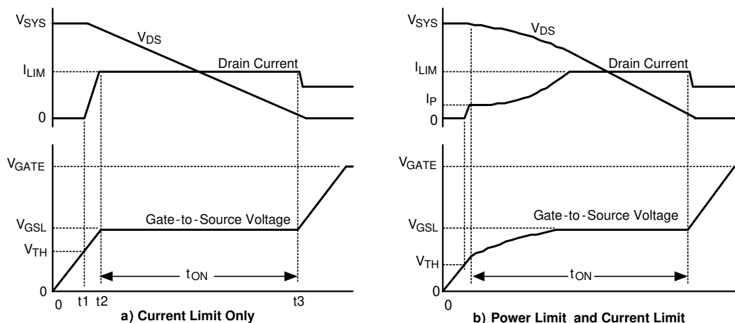
9-5. MOSFET Power Up Waveforms
