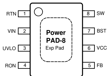
✎ 5-1. DDA Package 8-Pin SO PowerPAD Top View
