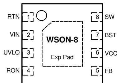
✎ 5-2. NGU Package 8-Pin WSON Top View
