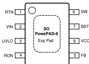
图 5-1. DDA Package 8-Pin SO PowerPAD Top View
