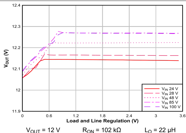
8-4. Load and Line Regulation Performance
