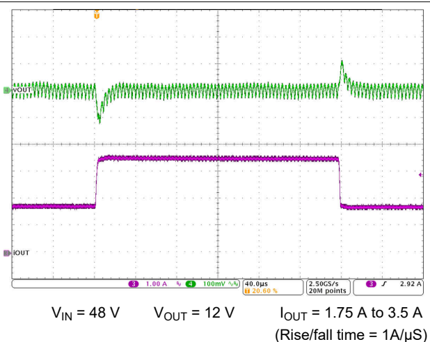
8-5. Load Step Response
