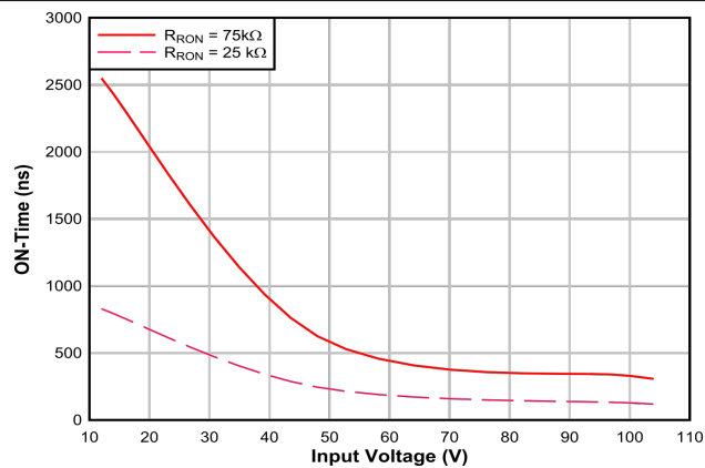
6-8. COT On Time Versus V_{IN}
