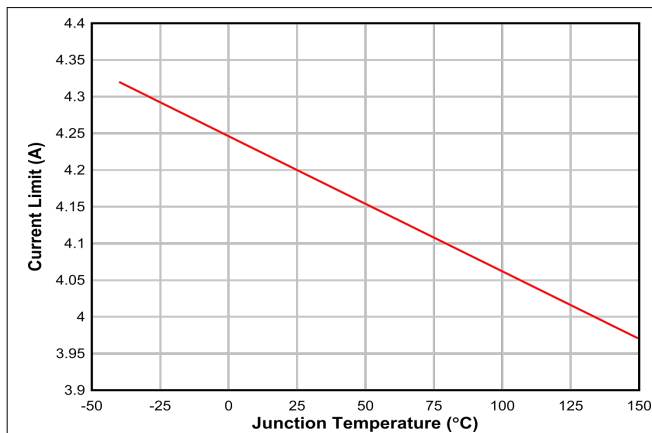
6-7. Peak Current Limit Versus Temperature
