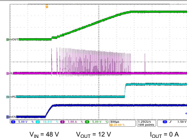
8-6. No-Load Start-Up with EN/UVLO
