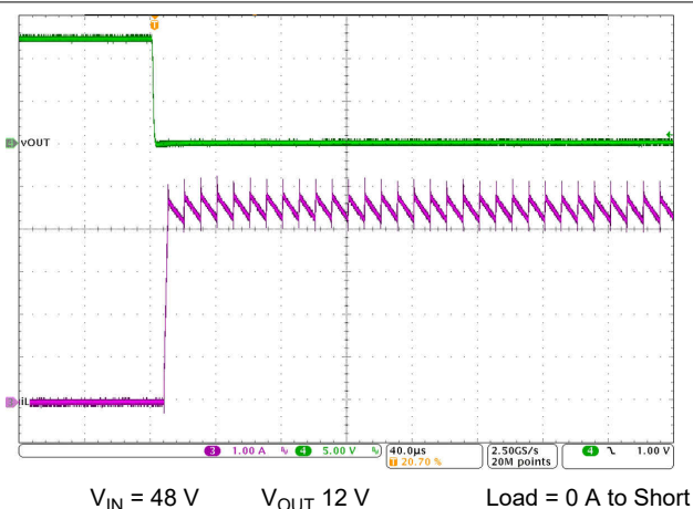
8-7. Short Circuit Applied
