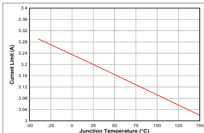
FIG 7-7. Peak Current Limit Versus Temperature
