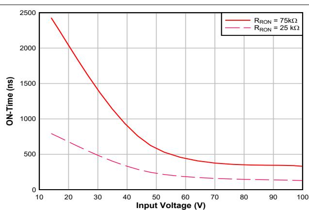
FIG 7-8. COT On Time Versus V_{IN}
