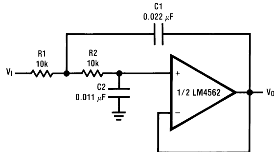
Figure 119. Second-Order High-Pass Filter (Butterworth)
