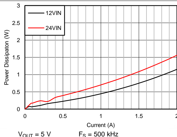
Figure 56. Power Dissipation at 85°C Ambient Temperature
