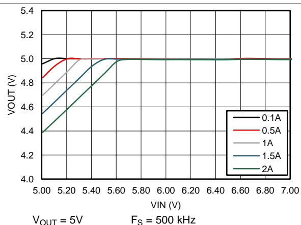
Figure 10. Dropout Curve
