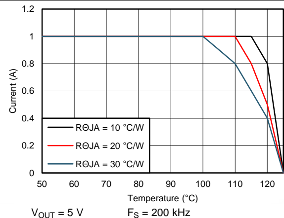
Figure 70. Derating Curve
