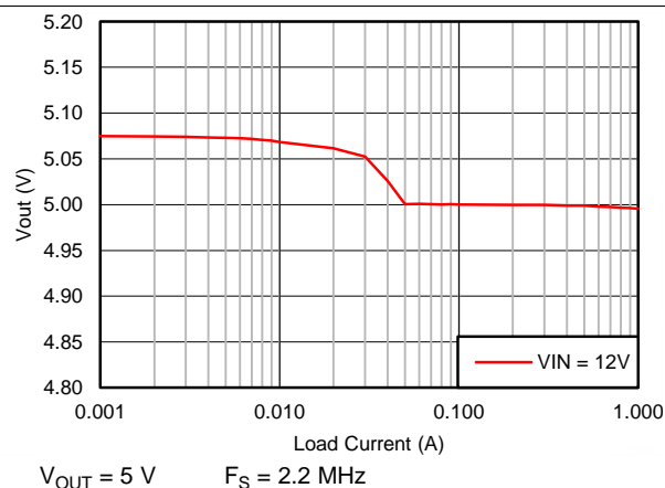
Figure 11. V_{OUT} Regulation
