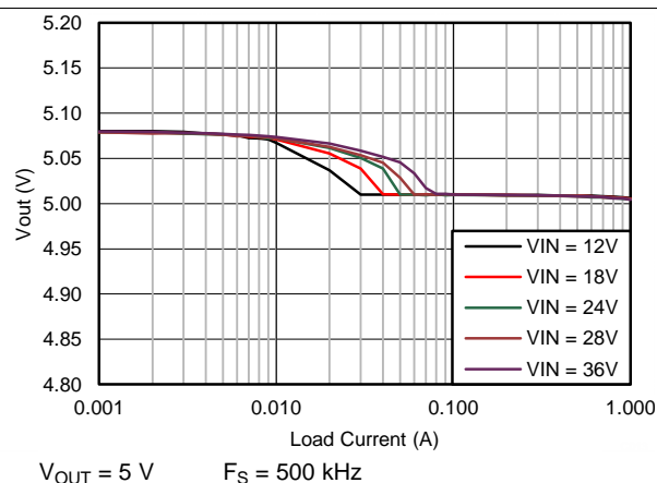
Figure 9. V_{OUT} Regulation
