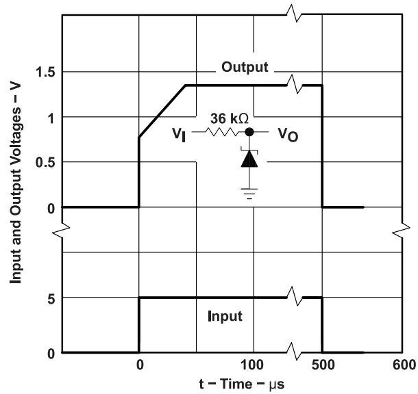
Figure 9. Transient Response
