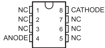
D, PS, PW or LP 8-Pin SOIC, SOP, TSSOP or TO-226 Top View
