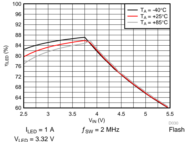
Figure 46. LED Efficiency vs Input Voltage
