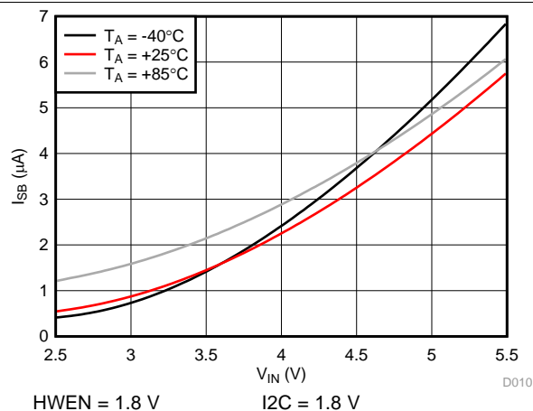
Figure 23. Standby Current vs Input Voltage
