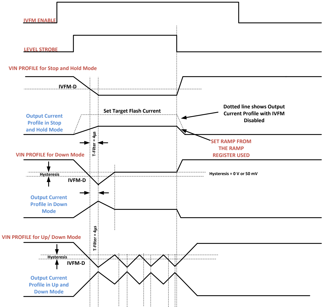
Figure 30. IVFM Modes
