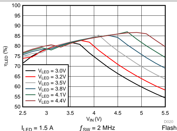
Figure 38. 4-MHz LED Efficiency vs Input Voltage
