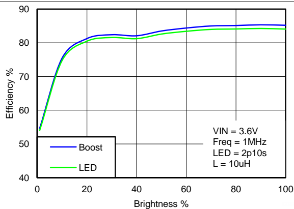
Figure 21. Boost and LED Efficiency
