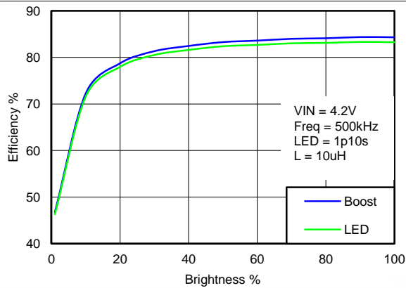
Figure 19. Boost and LED Efficiency
