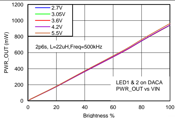
Figure 62. PWR_{IOUT} Across V_{IN}
