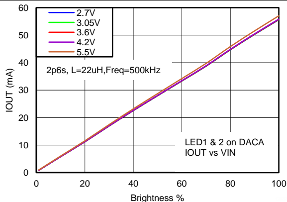
Figure 61. I_{OUT} Across V_{IN}
