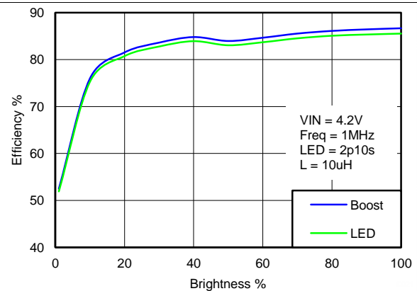
Figure 22. Boost and LED Efficiency
