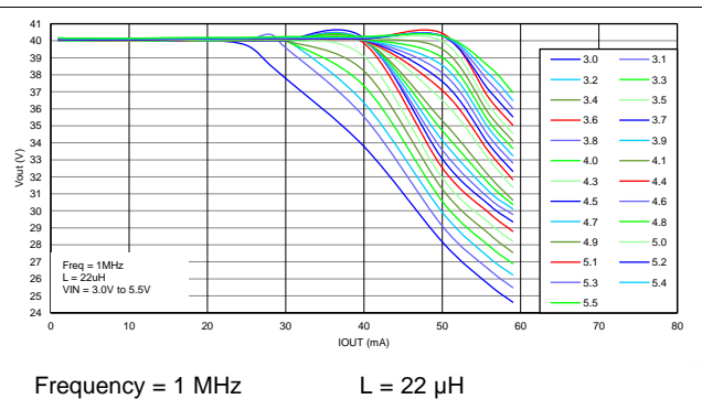
Figure 91. Maximum Boost Output Power vs V_{IN}
