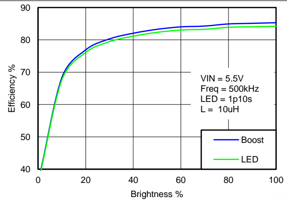
Figure 20. Boost and LED Efficiency
